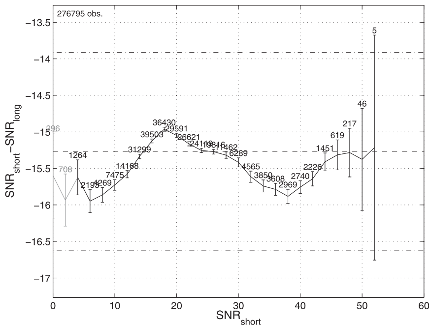
FIG. 9. As in Fig. 8, but between SNR_{SM} and SNR_{LM} (level 1) as function of SNR_{SM} (level 1).
