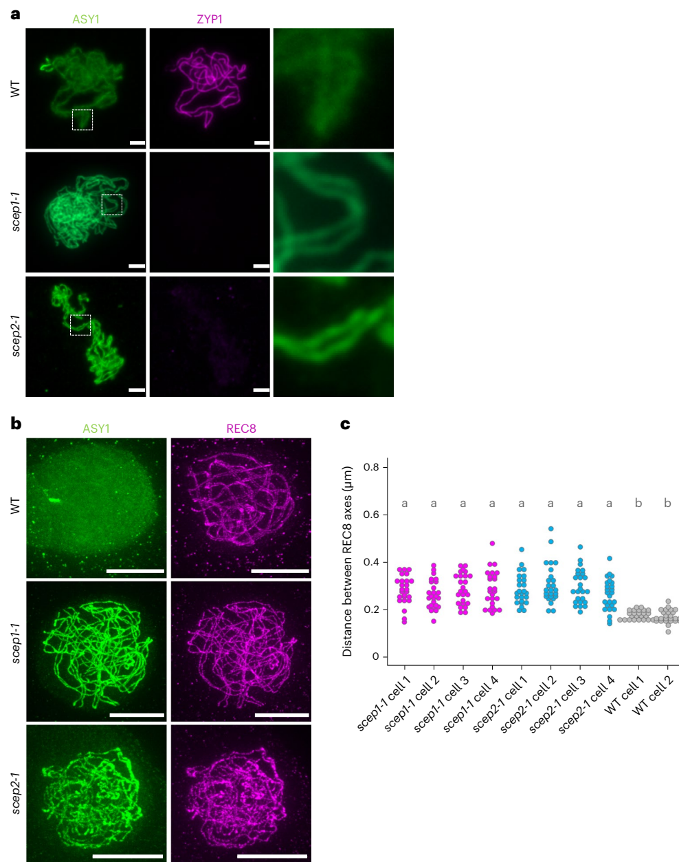
Fig. 2 | ZYP1 is not loaded in scep1 and scep2 mutants. a , Immunolocalization of ZYP1 and ASY1 in WT, scep1-1 and scep2-1 male meiocytes (standard-resolution microscopy). Scale bars, 2 \mu\text{m} . b , Immunolocalization of ASY1 (green) and REC8 (magenta) in WT, scep1-1 and scep2-1 male meiocytes analysed with STED
