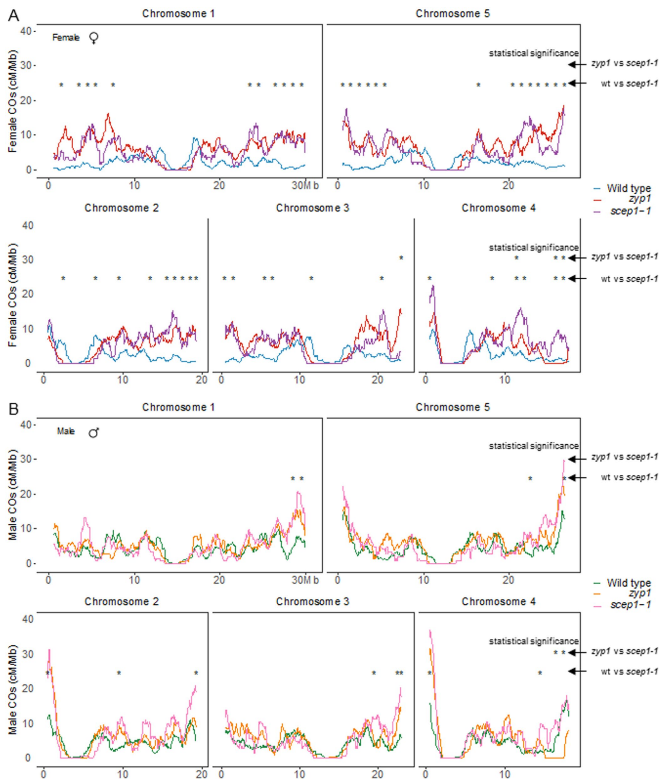
Extended Data Fig. 3 | The distribution of COs along the five chromosomes. The distribution of COs along chromosomes in female (A) and male (B) wild type, zyp1 and scep1-1 . The centromeric and pericentromeric regions are indicated by gray and blue shading, respectively. Analysis is done with 1-Mb windows and 50-kb sliding steps. For pericentromeric regions and each non-overlapping 1-Mb
