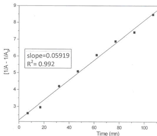
Figure 4. Photodegradation kinetics of maneb 5 \times 10^{-5} M in dichloromethane Constant rate k = 272.7 \text{ mol}^{-1} \cdot \text{L} \cdot \text{min}^{-1} . Half-life t_{1/2} = 73 mn. Second order kinetics. Correlation coefficient, R^2 = 0.992 .
