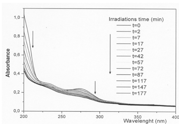
Figure 2. Absorption spectra of 5 x 10 -5 M solution of maneb in water before and after irradiation Broad band absorption with a peak at 275 nm and a shoulder at around 230 nm.
