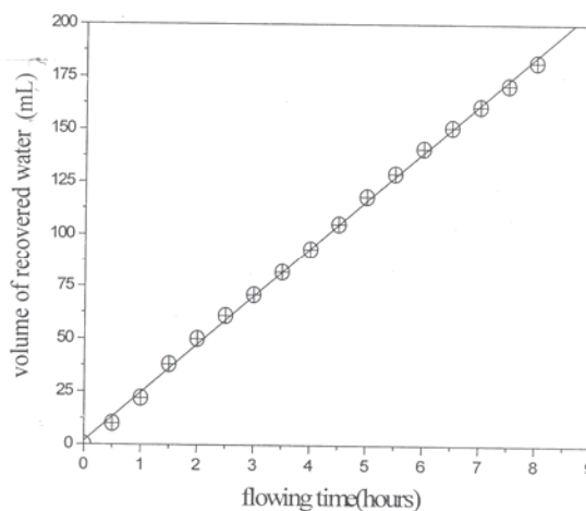
Figure 6. Permeability of sand to distilled water
