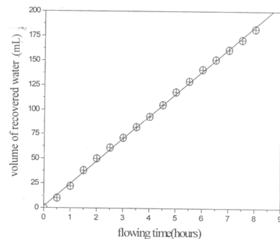
Figure 6. Permeability of sand to distilled water Height of the column, 50 cm. Diameter of the sand, 0.25 mm. Rate of water flow, 0.5 mL/min. Period of recovery, 8 hours.
