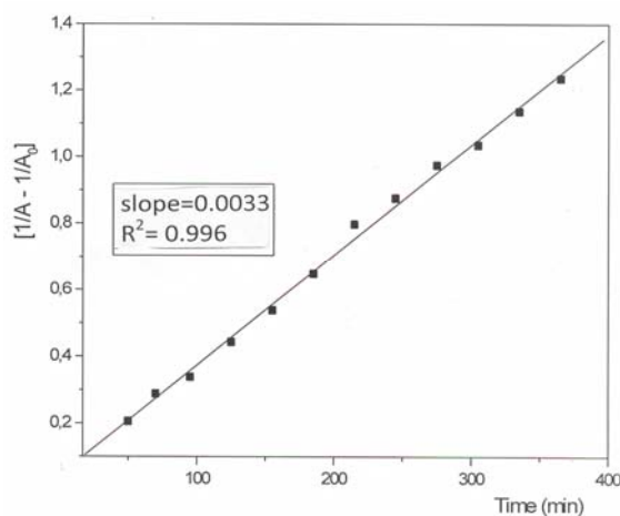
Figure 5. Photodegradation Kinetics of propanil 2.5 \times 10^{-5} M in water Constant rate k = 30.57 \text{ mol}^{-1} \cdot \text{L} \cdot \text{min}^{-1} . Half-life t_{1/2} = 1574 mn (26 \frac{1}{2} h). Second order kinetics. Correlation coefficient, R^2 = 0.996 .
