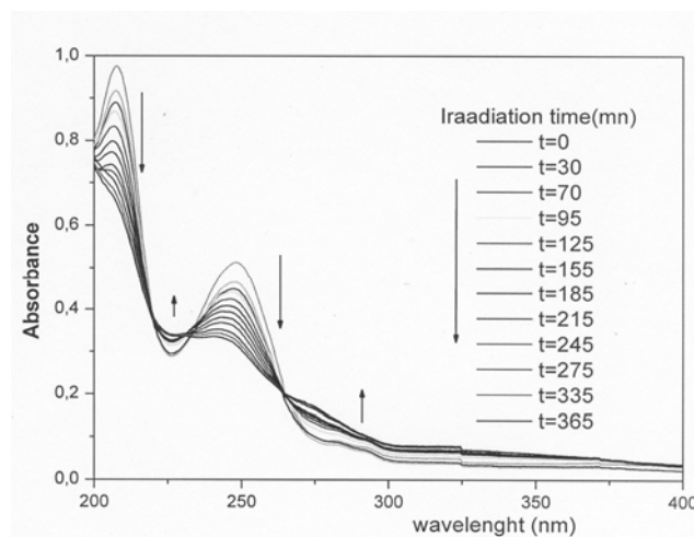
Figure 3. Absorption spectra of a 2.5 x 10 -5 M solution of propanil in water before and after irradiation Broad band between 200 and 400 nm with two peaks at 208 nm and at 249 nm for propanil. A band for an unknown photoproduct between 265 and 400 nm.
