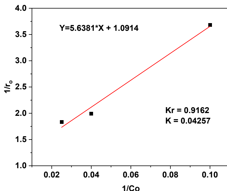
Figure 13. Langmuir–Hinshelwood kinetic plot for the photocatalytic decolorization of methyl blue.
