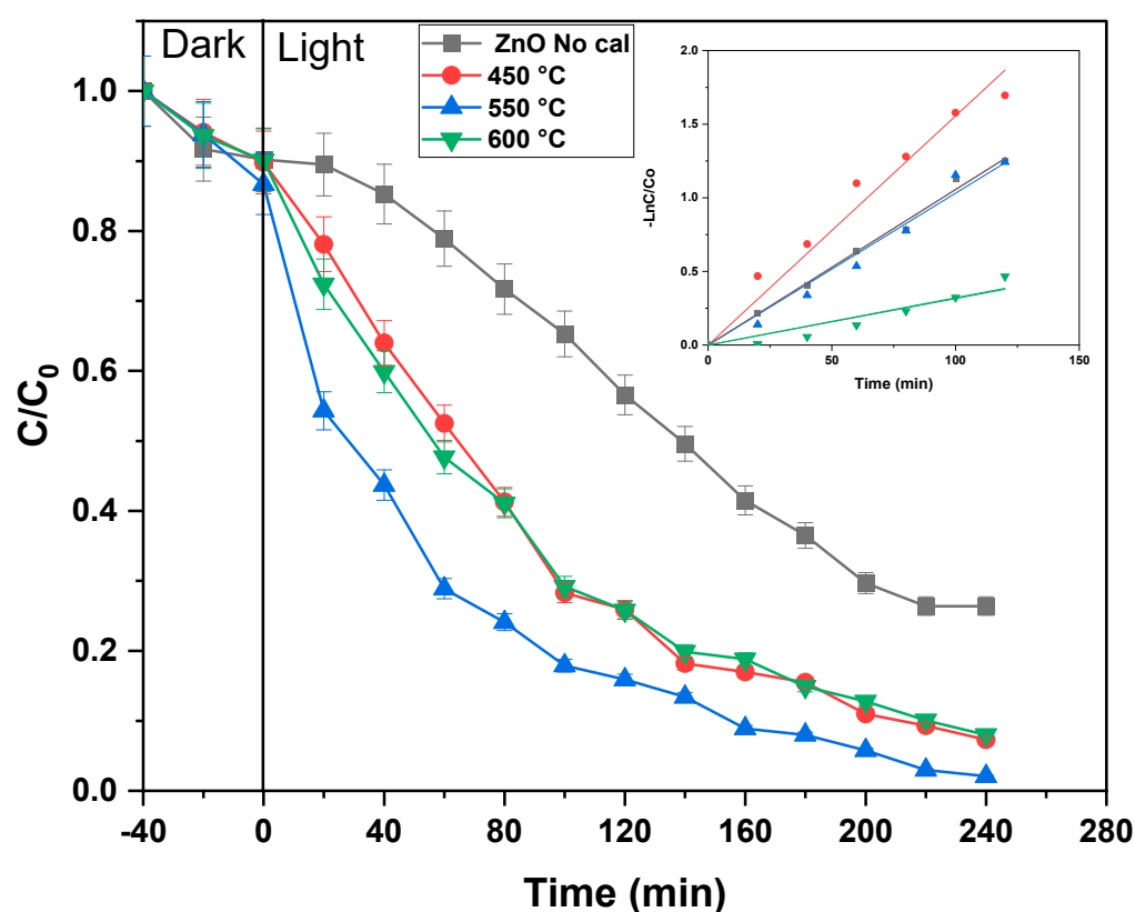
Figure 6. Effect of calcination temperature on the photocatalytic activity of ZnO for the photocatalytic degradation of MB (neutral pH, catalyst 1 g/L, [MB] = 10 mg/L).
