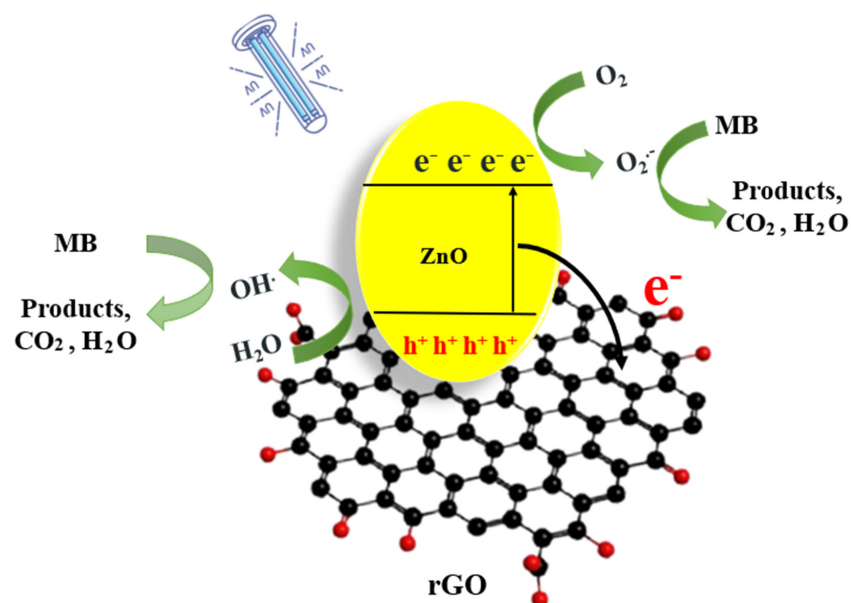
Figure 14. The photodegradation mechanism of methylene blue.
