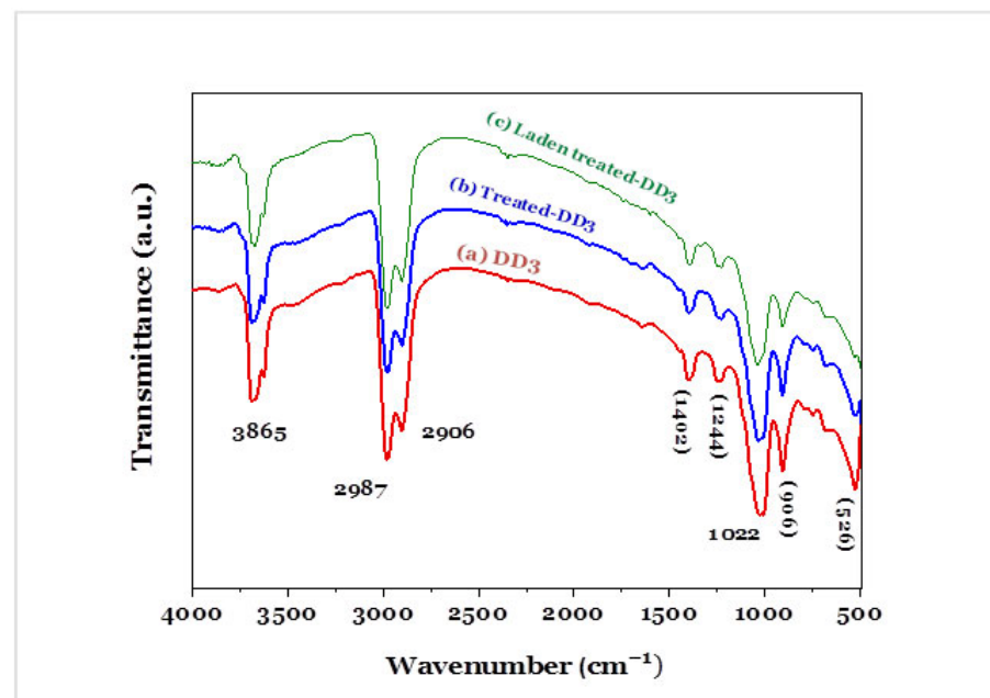
Figure 4. FTIR spectrum of (a) DD3, (b) treated-DD3, and (c) treated-DD3 after adsorbing MB dye.
