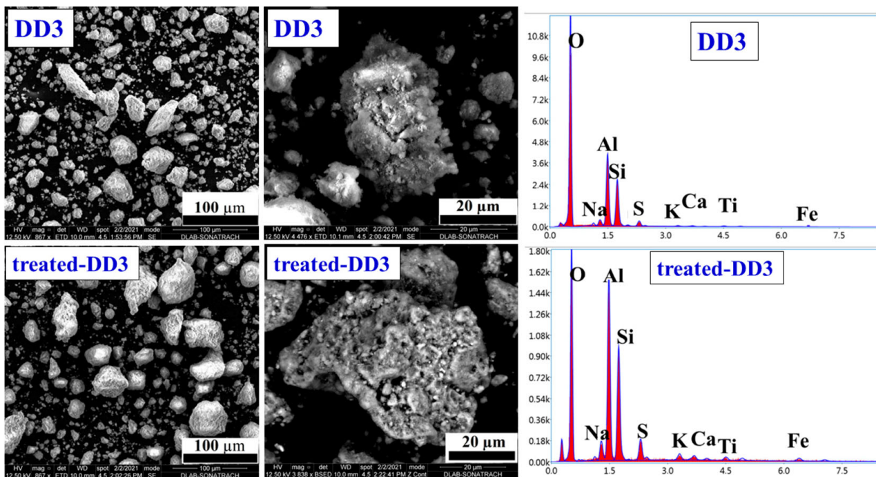
Figure 2. SEM images and EDS data of the DD3 and treated-DD3 kaolinites.
