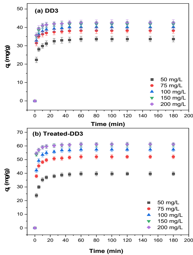
Figure 6. Effect of contact time and initial concentration of MB on the adsorption capacity of (a) DD3 and (b) treated-DD3 ( m/V = 1 \text{ g/L} , 25 \pm 3 \text{ }^\circ\text{C} , and unadjusted pH).
