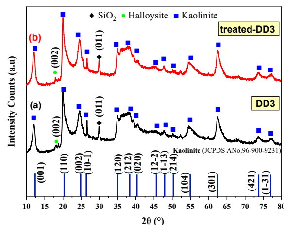
Figure 1. XRD data of (a) DD3 and (b) treated-DD3 kaolinites.
