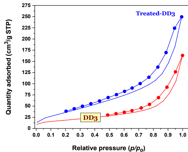
Figure 3. Nitrogen adsorption/desorption isotherms at 77 K of DD3 and treated-DD3 kaolinites.
