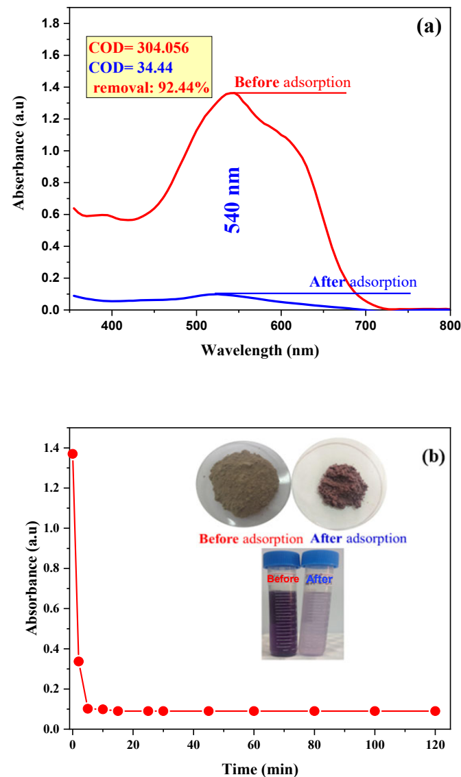
Figure 8. (a) COD values of the BM-wastewater effluents before and after adsorption on treated-DD3; and (b) Effect of contact time of BM-wastewater decolorization on treated-DD3 (pH of the effluent, m/V = 1 g/L, and 25 \pm 3 °C).
