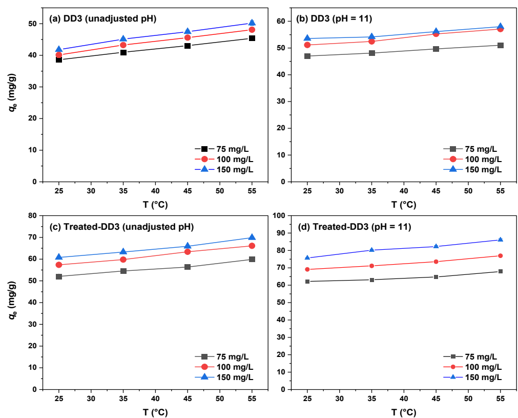
Figure 7. Effect of temperature on the adsorption capacity of the MB dye onto (a,b) DD3 and (c,d) treated-DD3 at different solutions' pH and initial dye concentrations.
