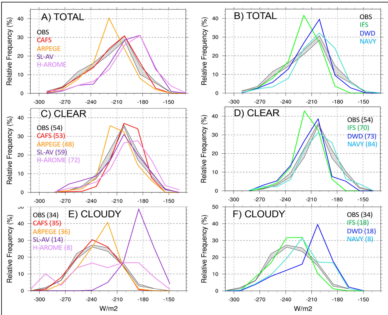
Figure 3. Probability Distribution Functions (PDFs) of model hourly averaged upwelling surface longwave fluxes, in units of Wm^{-2} , using 1 h to 2 day lead times. (A and B) Using all hourly samples. (C and D) Using hourly clear-sky samples. (E and F) Using hourly cloudy samples. The gray shading shows the range of the observed distributions using hourly averaged measurements from the 4 MOSAiC sites. Individual model distributions shown with colored lines as indicated in the legends. The numbers in the legends for the clear and cloudy distributions show the percent of the total sample used in the PDFs.
