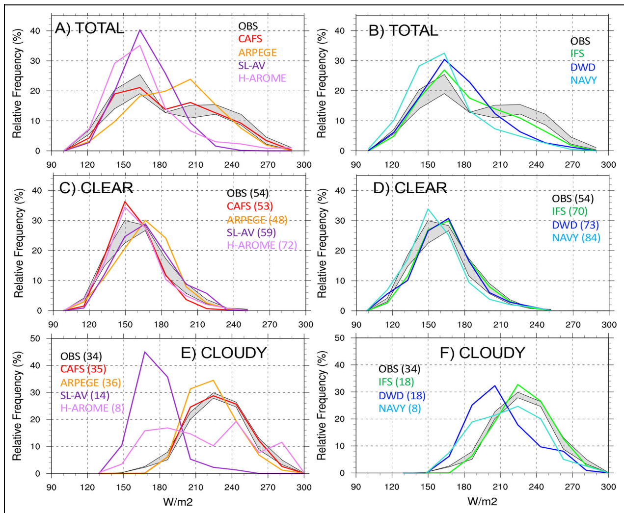
Figure 2. Probability Distribution Functions (PDFs) of model hourly averaged downward surface longwave fluxes, in units of Wm^{-2} , using 1 h to 2 day lead times. (A and B) Using all hourly samples. (C and D) Using hourly clear-sky samples. (E and F) Using hourly cloudy samples. The gray shading shows the range of the observed distributions using hourly averaged measurements from the 4 MOSAiC sites. Individual model distributions shown with colored lines as indicated in the legends. The numbers in the legends for the clear and cloudy distributions show the percent of the total sample used in the PDFs.
