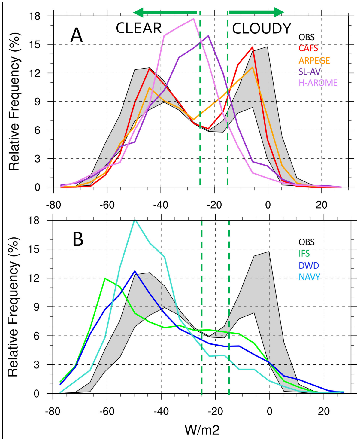
Figure 1. Probability Distribution Functions (PDFs) of model hourly averaged net surface longwave fluxes, in units of Wm^{-2} , using 1 h to 2 day lead times. The gray shading in both plots shows the range of the observed distributions using hourly averaged measurements from the 4 MOSAiC sites. Individual model distributions (shown with colored lines as indicated in the legends) are separated into 2 plots in order to clearly distinguish differences; (A) CAFS, ARPEGE, H-AROME, SL-AV; (B) IFS, DWD, NAVY. Clear-sky periods are defined in this article as net longwave fluxes less than -25 Wm^{-2} . Cloudy sky periods defined as net longwave fluxes greater than -15 Wm^{-2} .
