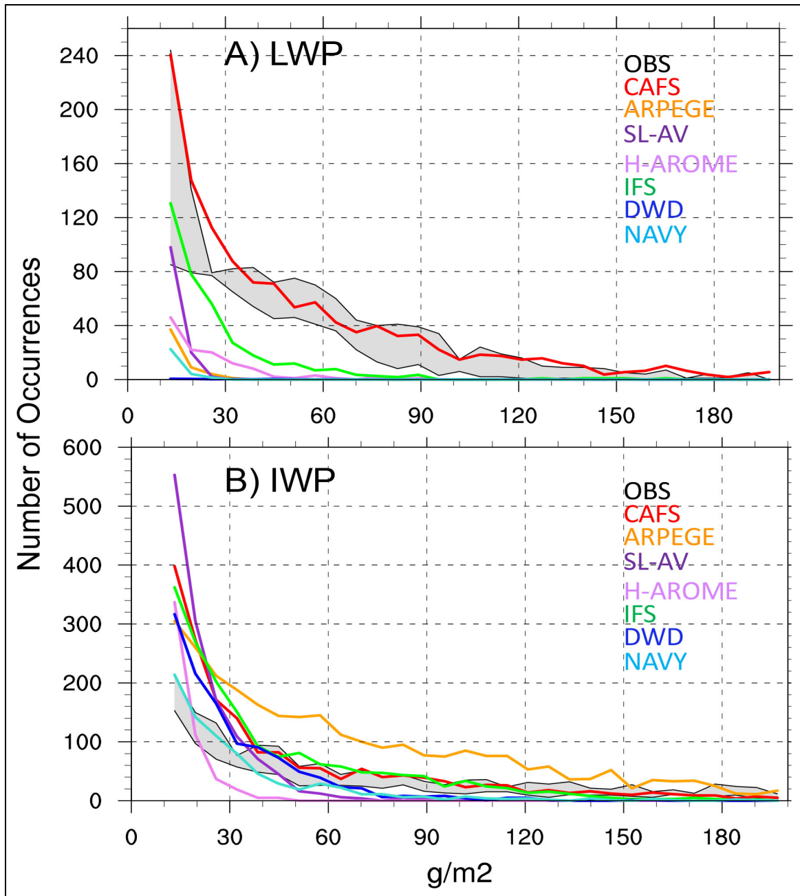
Figure 4. Number of occurrences of modeled (A) LWP greater than 10 \text{ gm}^{-2} and (B) IWP greater than 10 \text{ gm}^{-2} over the winter season. The gray shading shows the observed range within each hour using 1 min averages. Individual model distributions using the first 24 hours of each simulation shown with colored lines as indicated in the legends.
