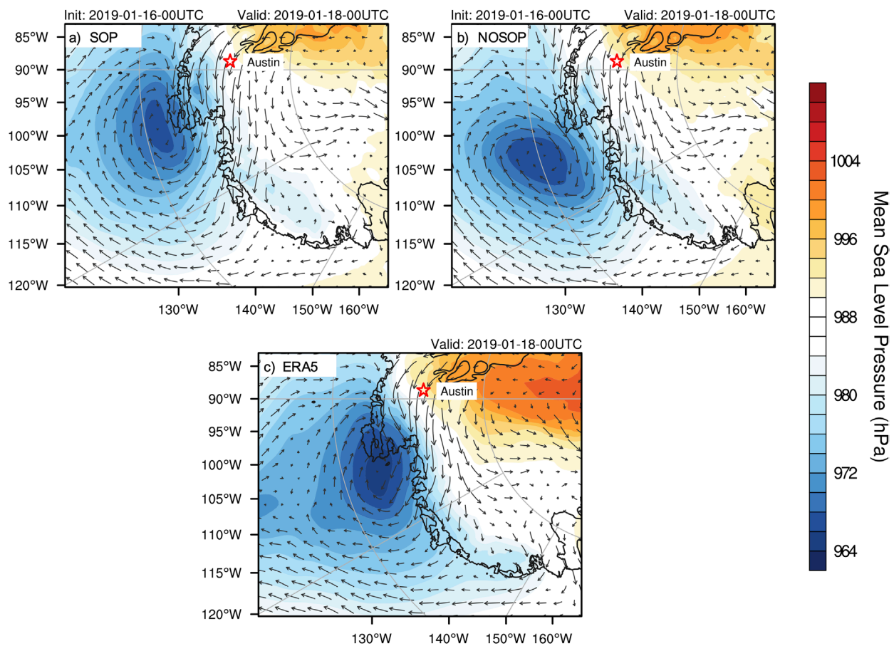
Fig. 9. Sea level pressure (shaded, hPa, scale to right) and surface winds (vectors) from 48-h (a) SOP forecast and (b) no-SOP forecast and from (c) the ERA5 global reanalysis, valid 0000 UTC 18 Jan 2019. Coast of West Antarctica shown and Austin AWS marked.
