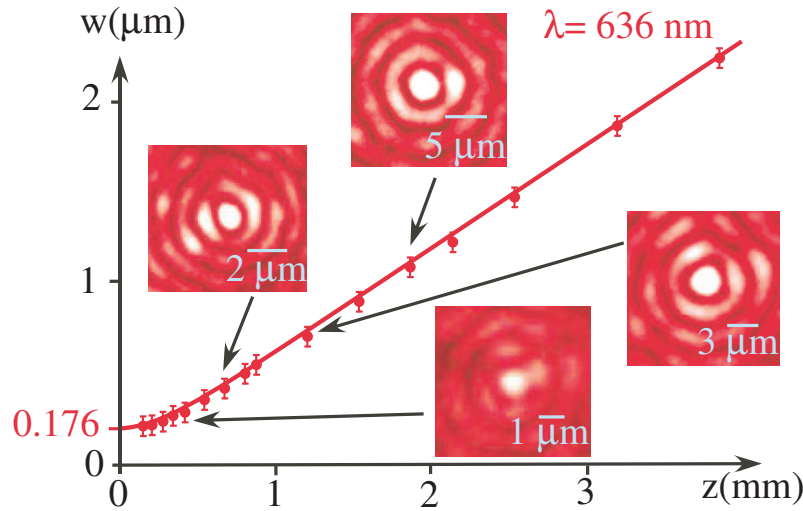
Figure 4. Variation in the size of the Arago–Poisson spot with the distance from the occulting disk (diameter d = 0.6 mm). As the distances reduce, the size tends to 176 nm. The experimental uncertainty reads in the error bars. The solid line corresponds to the theoretical curve of Equation (1). Inserts, pictures of the Arago–Poisson spots corresponding to the experimental points. Note that the scale changes for each insert.
