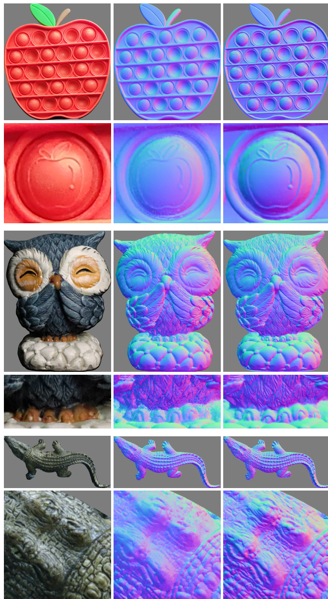
SDM-UniPS [Ikehata (2023)] SDM-UniPS [Ikehata (2023)] Our Universal Transformer
