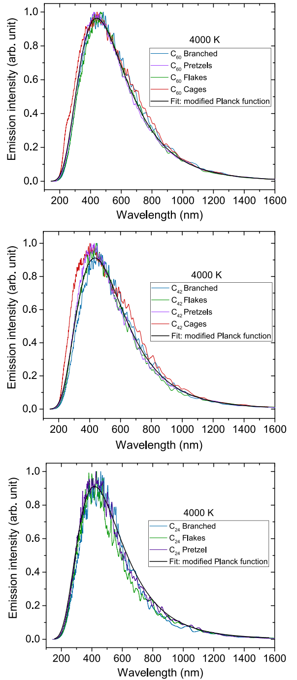
Fig. 10. Emission spectra from samples containing around 1000 isomers. The simulated histogram emission spectra has been broadened by a Gaussian function with FWHM = 10^5 \lambda^2 / \text{nm} . The fit function is a modified Planck function expressed as [\lambda^8 (\exp(\frac{hc}{k_B T \lambda}) - 1)]^{-1} .
