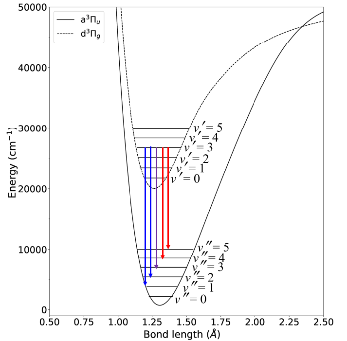
Fig. 3. Ground ( a^3\Pi_u ) and excited ( d^3\Pi_g ) electronic states of the Swan system of 12 C 2 . The \Delta v = +1 and +2 transitions are in blue, the \Delta v = 0 transition is in purple, and the \Delta v = -1 and -2 transitions are in red.
