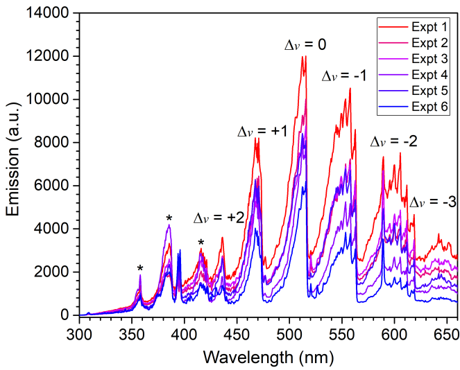
Fig. 2. UV-Vis emission spectra of shock-processed C 60 showing C 2 features and a broad continuum. The spectra were recorded under different experimental conditions, as reported in Table 1. The C 2 vibronic bands were labeled according to the Herzberg (1995) notation: \Delta v = v' - v'' ; v' and v'' refer to the upper and lower vibrational levels, respectively. The spectral features below 420 nm flagged with an asterisk (*) were assigned to contaminants.
