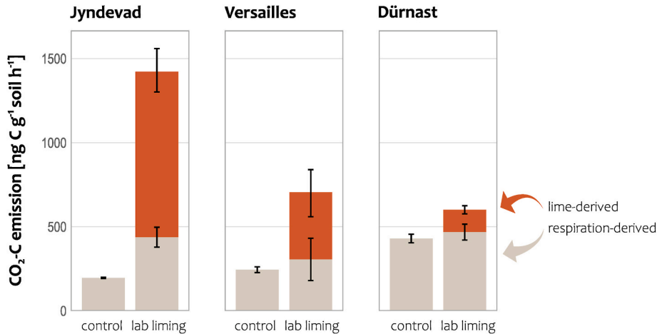
Fig. 2. Mean absolute CO 2 -C emissions ± standard deviation from the control soils per site, incubated without (i.e. control) and after laboratory addition of lime (i.e. lab liming). The colours indicate the source of CO 2 -C emissions as differentiated based on the δ 13 C signatures (orange: lime-derived, grey: respiration-derived).
