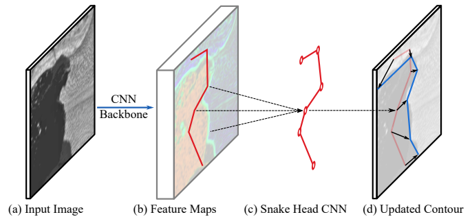
Fig. 1. High-level overview of our deep active contour model for delineating calving fronts. First, the backbone network takes the input image (a) and derives feature maps. Then, a sample is taken from these feature maps at the position of each vertex (b). These features are evaluated by the Snake Head CNN (c) which predicts offsets for each vertex. Finally, the offsets are applied to update the contour (d). This process is repeated multiple times.
