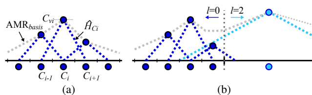
Figure 4: AMR basis reconstruction by Wald et al. [WBUK17]. (a) For structured data, basis function reconstruction is equivalent to trilinear interpolation. (b) Reconstruction at a l = 0 to l = 2 level transition. The reconstructed function is C^0 -continuous and adaptive, yet not interpolative.
