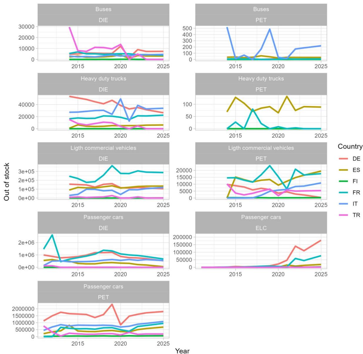
Vehicles out of the stock. Source Eurostat.
