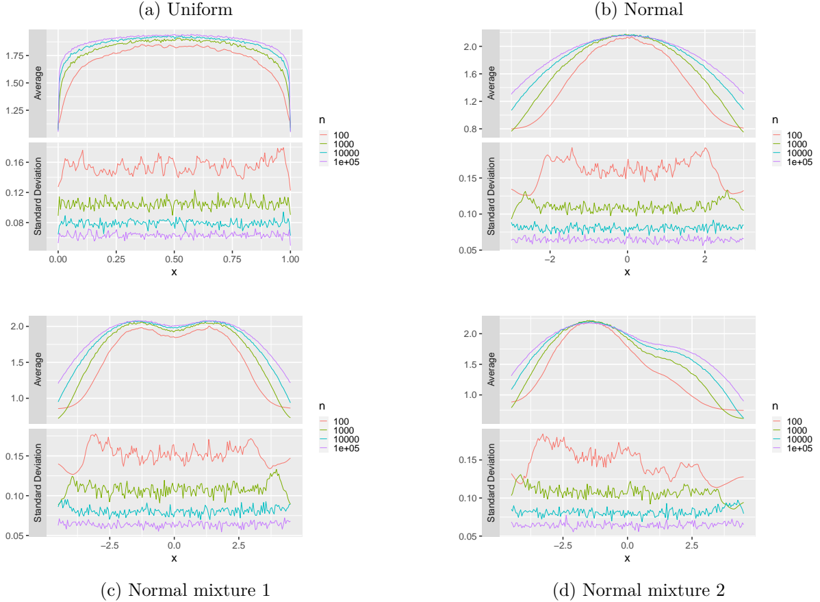
Figure 3: Numerical examples illustrating the setting of Corollary 8. Here N = 200 samples of sizes n^k , with k \in \{2, 3, 4, 5\} , were simulated according to a uniform distribution, a standard normal distribution, and mixtures of normal distributions with variances equal to 1, means equal to -1.5 and 1.5 , and mixture coefficients equal to 0.5 and 0.5 (mixture 1) and 0.9 and 0.1 (mixture 2). The pointwise average and standard deviation of \mathbb{E}[h_{\mathcal{T}}(x) | X_1, \dots, X_n] were evaluated on the N samples at 200 equally spaced points x that extend over [0, 1] (uniform case), over [-3, 3] (standard normal case) and over [-4.5, 4.5] (mixture cases).
