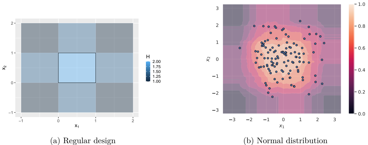
Figure 4: Numerical example illustrating the setting of Theorem 9 showing that the scoring function admits axis-aligned discontinuities in regions outside the support of the distribution. Here are represented in subfigure (a) the limit function of Theorem 9 for the regular design (21) over [0, 1]^2 , and in subfigure (b) the scoring function (normalized between 0 and 1) that results from applying the isolation forest algorithm to a sample of size n = 120 drawn from a standard multivariate normal distribution over \mathbb{R}^2 .
