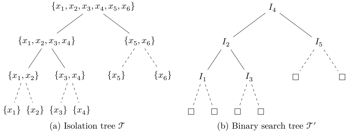
Figure 1: An isolation tree \mathcal{T} is represented in (a) and its associated binary search tree \mathcal{T}' = (\tilde{\tau}^{-1} \circ \iota)(\mathcal{T}) is represented in (b). Edges to the leaves are represented with dashed lines and the leaves of the binary search tree \mathcal{T}' are represented with empty boxes.
