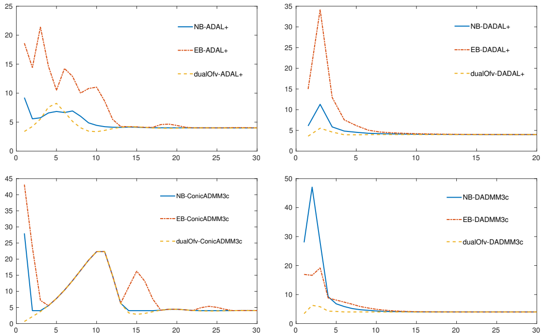
Figure 1: Evolution of the computed bounds on the instance johnson8_2_4 .
