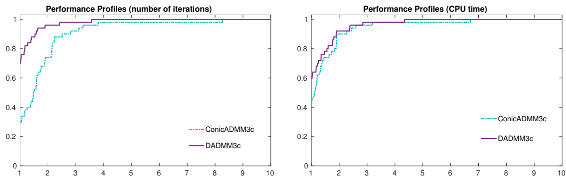
Figure 3: Comparison between ConicADMM3c and DADMM3c on DIMACS instances [8].
