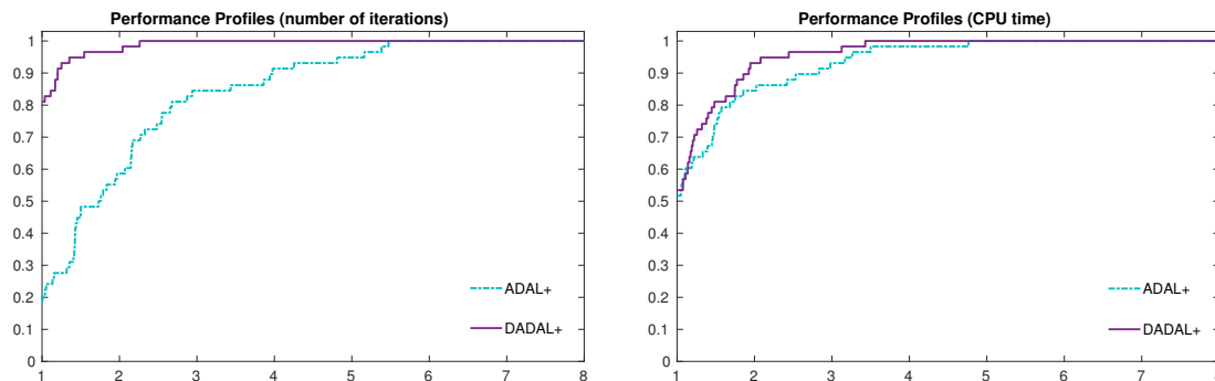
Figure 2: Comparison between ADAL+ and DADAL+ on DIMACS instances [8].
