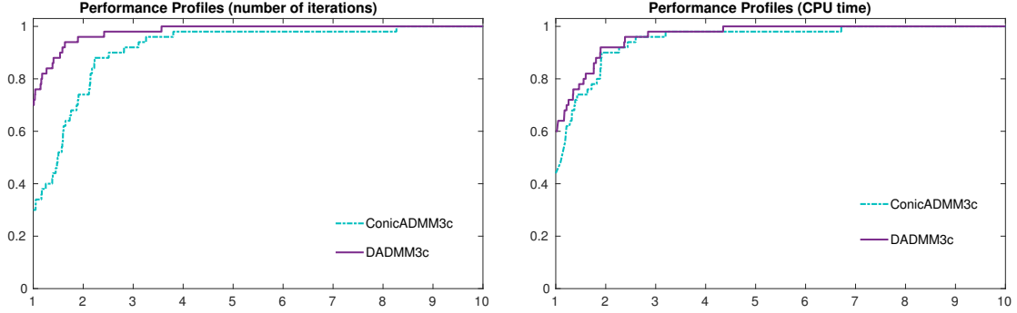
Figure 3: Comparison between ConicADMM3c and DADMM3c on DIMACS instances [8].
