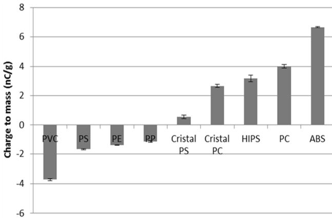
Fig. 6. Charge to mass ratio for nine types of particles passed through PVC cylinder tribocharging device.
