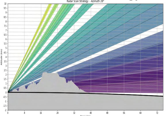
PPI scan strategy
