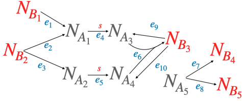
Figure 1: \mathcal{H}^{O_0} , concepts and roles in \Sigma_0 are in red.
