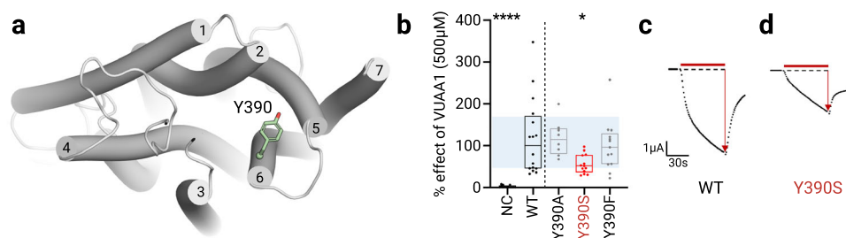
Fig. 3 | Electrophysiological characterization of Orco mutants in the contact region. a Top view of the entry highlighting the position of Y390. b Boxplot showing the current induced by 500 μM of the ligand VUAA1 and measured by TEVC recordings on DmelOrco WT and mutants expressed in Xenopus oocytes. The lower bound of the box plot represents the first quartile, while the upper bound represents the third quartile. The centre corresponds to the median. The blue area is a projection of the first and third quartiles of the WT box plot. n = 13 recordings
