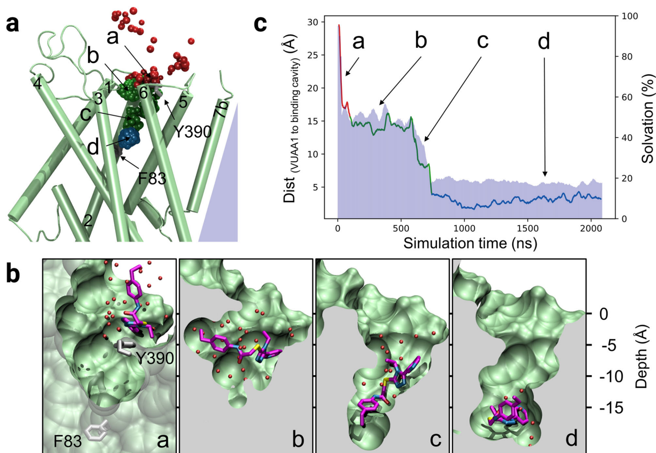
Fig. 2 | Stepwise translocation of VUAA1 into DmelOrco model in MD simulations. a Prototypical trajectory of VUAA1 binding event. The Orco monomer is shown in green. F83 and Y390 labels give their localization. The VUAA1 center of mass is represented by beads colored from red to blue according to the simulation time. a–d are sequential positions of VUAA1 progressing toward the binding site, from contact to Orco, entry, vestibule and binding to the internal cavity, respectively. b Close view of the progression of VUAA1 inside the Orco monomer corresponding to the positions a–d . Carbon atoms of VUAA1 are colored purple and the sulfur atom in yellow. Carbon atoms of F83 S2 and Y390 S6 are in grey and water
