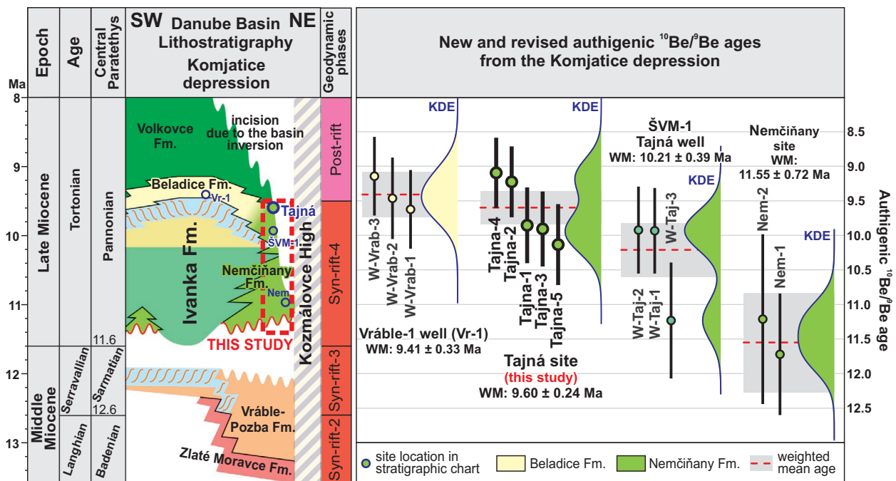
Fig. 7. Authigenic ^{10}\text{Be}/^9\text{Be} dating results and their stratigraphic context. Ages for the Vrable-1 well, ŠVM-1 Tajná well and the Nemčiňany outcrop are from Šujan et al. (2016). Weighted mean ages (WM) and Kernel Density Estimation (KDE) are established using the KDX software by Spencer et al. (2017), with 1\sigma as uncertainties. See Fig. 1D for the stratigraphic chart explanations.
