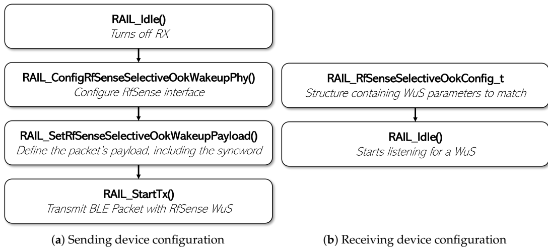
Figure 10: WuR (RFSense) usage on an EFR32BG22.
