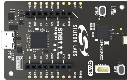
(a) BG-22 Explorer Kit
