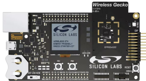
(b) EFR32xG22 Wireless Gecko Starter Kit
