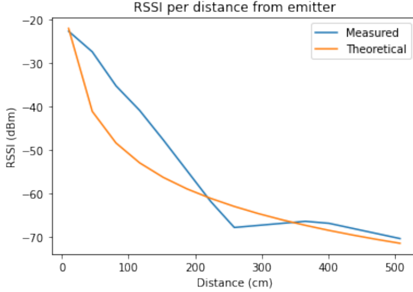
Figure 11: RSSI measurements.
