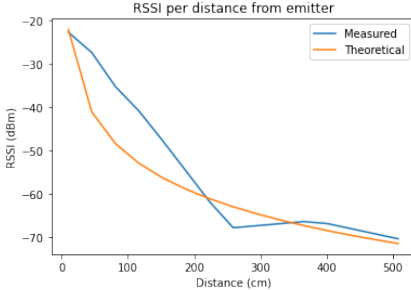
Figure 11: RSSI measurements.
