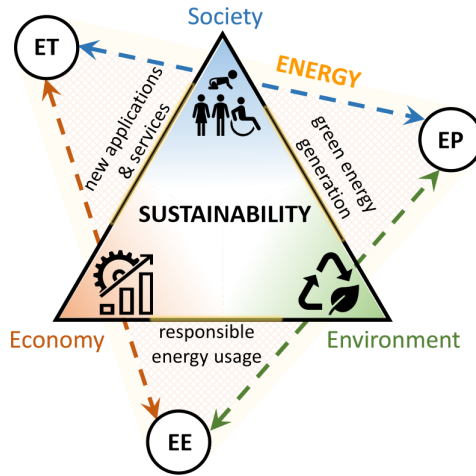
Figure 1: Sustainability triangle [6].
