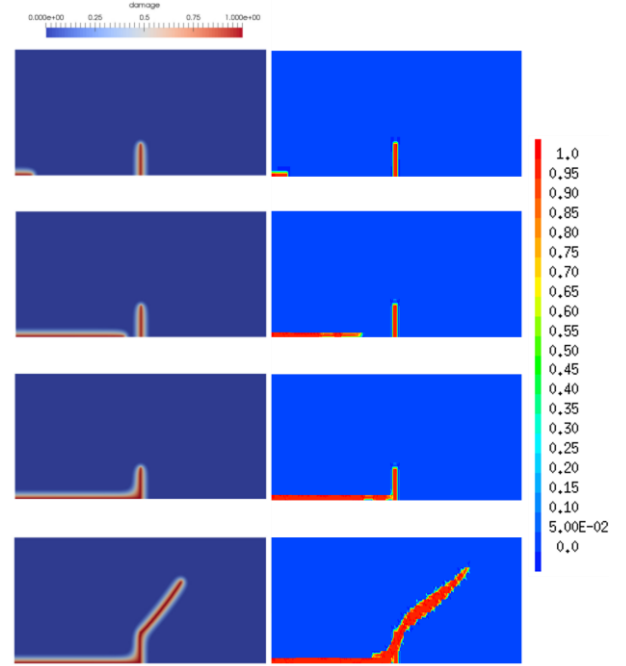
Figure 5: crack pattern left : after [14], right : our model
