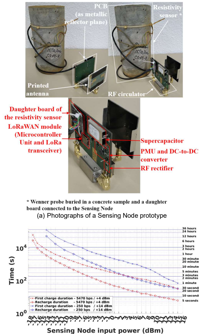
(b) Durations of the first charge ('x') and recharges ('o') against the conducted electromagnetic input power applied at the input of the rectifier of the Sensing Nodes, for a frequency of 868 MHz, and for two configurations of the wireless communication: transmission power of +4 dBm and data-rate of 5470 bps (dashed lines), and transmission power of +14 dBm and data-rate of 250 bps (dotted lines).
