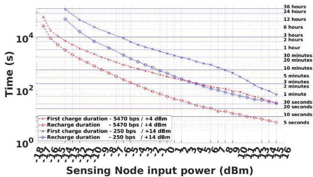
(b) Durations of the first charge ('x') and recharges ('o') against the conducted electromagnetic input power applied at the input of the rectifier of the Sensing Nodes, for a frequency of 868 MHz, and for two configurations of the wireless communication: transmission power of +4 dBm and data-rate of 5470 bps (dashed lines), and transmission power of +14 dBm and data-rate of 250 bps (dotted lines).
