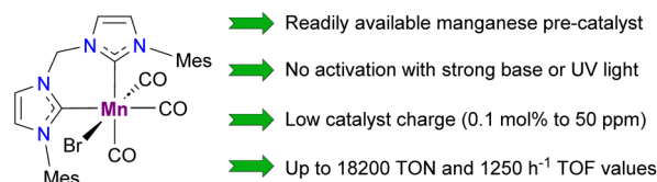
Scheme 1 Different types of cooperative bimetallic activation of organic molecules (top, dashed and dotted lines refer to activated/cleaved bonds in the substrate and non-covalent interactions, respectively) and the Mn(I) precursor used for catalytic intermolecular amine-borane dehydrogenation (bottom).
