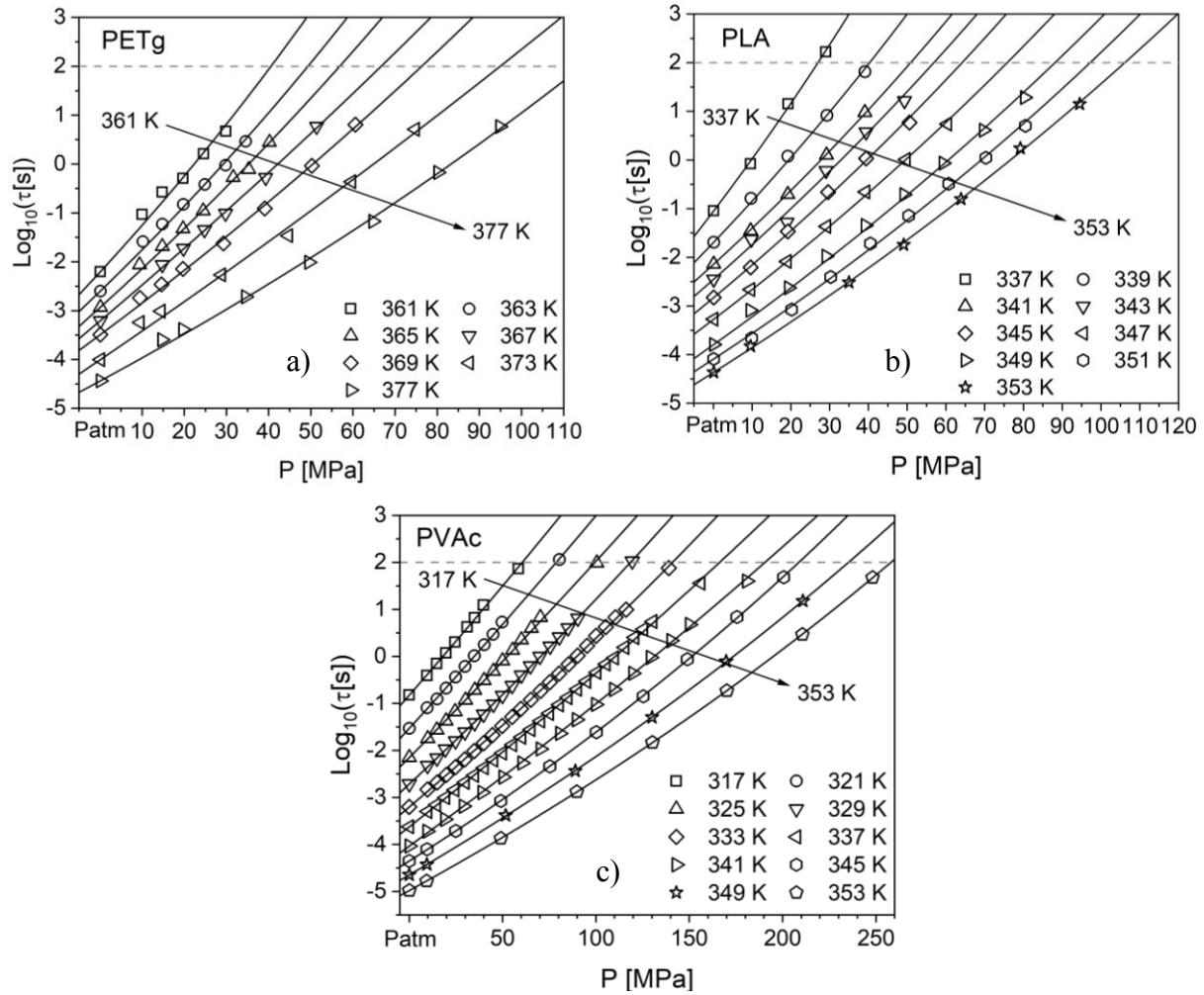
Figure 2. Pressure dependence of isothermal \alpha -relaxation time for a) PETg, b) PLA and c) PVAc. The black lines are the pressure VFT fits for each isotherm. The dashed grey lines correspond to isochrone \tau = 100 s, i.e. to the glass transition pressure P_g , analogous to the glass transition temperature T_g .
