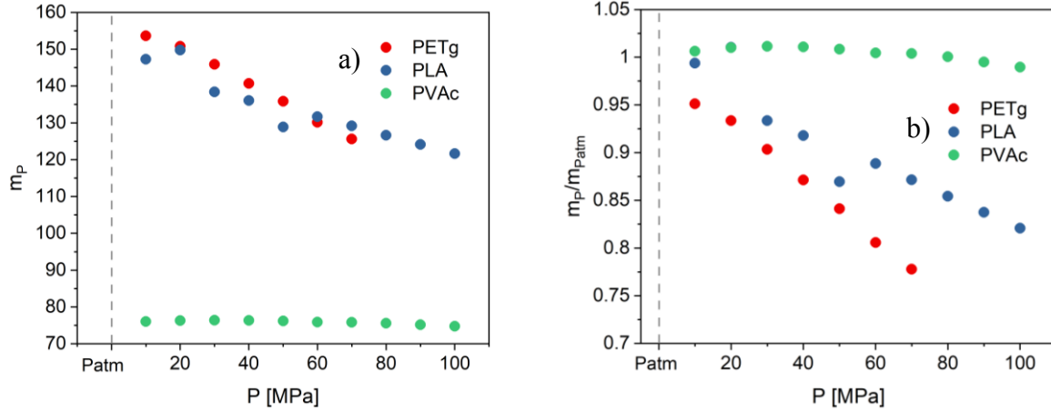
Figure 5. PETg in red, PLA in blue and PVAc in green. a) Isobaric fragility m_P as a function of pressure. b) Isobaric fragility normalized to the isobaric fragility at P_{\text{atm}} as a function of pressure.
