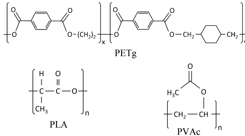
Figure 1. Structural unit of the polymers studied in this work. PETg have ratio of x = 2/3 and y = 1/3 .
