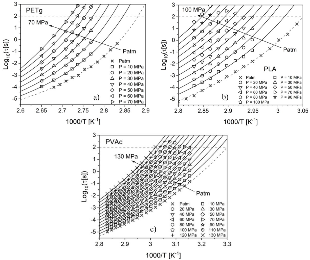
Figure 3. Temperature dependence of isobaric \alpha -relaxation time \tau for a) PETg, b) PLA and c) PVAc. The black lines are VFT fits of each isobar. The dashed black lines correspond to the VFT fit at P_{\text{atm}} . The dashed grey lines correspond to isochrone \tau = 100 s, i.e. to the glass transition temperature T_g .
