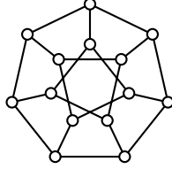
Figure 1: The generalized Petersen graph P(7, 2) .
