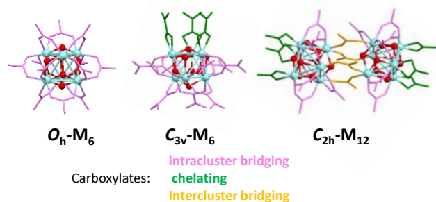
Figure 1. Topologies of [M_6O_4(OH)_4(O_2CR)_{12}]_n clusters ( M = Zr, Hf; n = 1 or 2 ).
