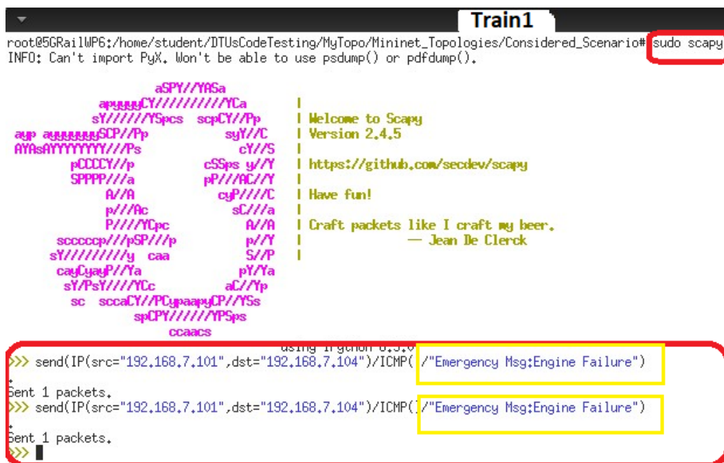
Figure 30. Scapy: packet creation.
