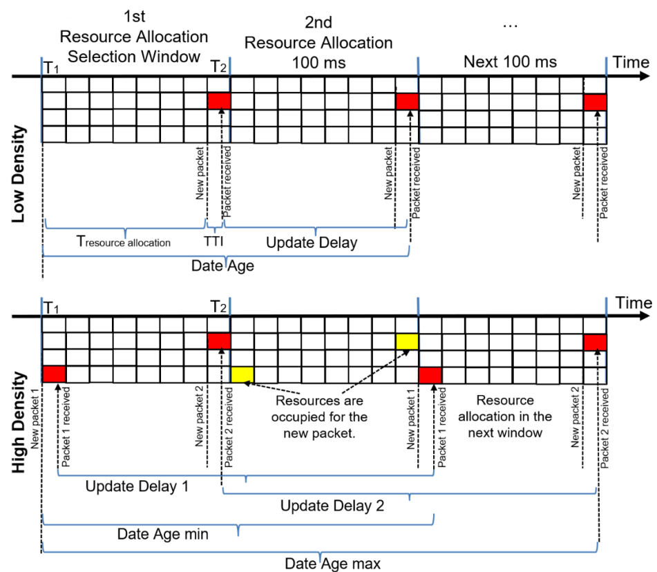
Figure 7. Update delay and date age for LTE-V2X.
