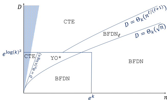
■ Figure 1 Regions of (n, D) where either of CTE, \text{Yo}^* , BFDN and BFDN _{\ell} has the best runtime guarantee. The runtime of algorithm \text{Yo}^* was simplified to improve readability. \ell must satisfy \ell \leq \text{cst}(\log k / \log \log k) . No trees defined in shaded region n \leq D . See Appendix A for details.
