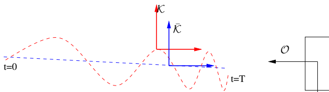
Fig. 4. \mathcal{K} is the current camera frame and \bar{\mathcal{K}} is the camera position obtained if the visual servoing velocity is applied without the walking constraints.
