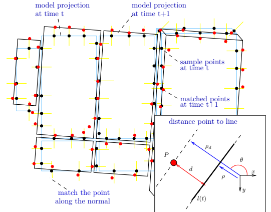
Fig. 3. Model-based tracking principle.
