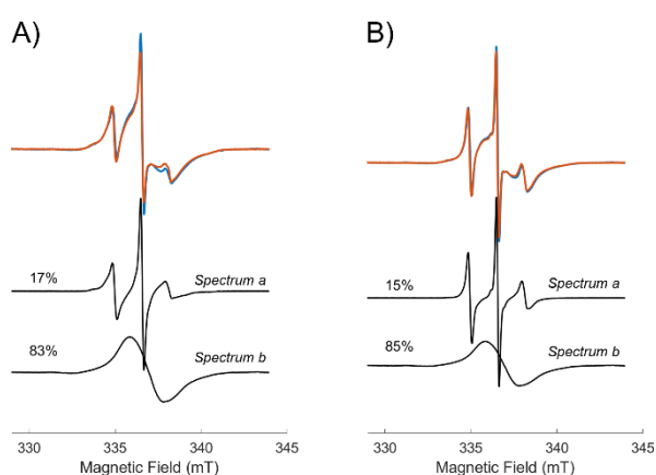
Figure 4. Cw X-band EPR spectra recorded at room temperature of labelled one electron reduced Homo sapiens CPR mutants A) FMNH*/Q157 pAzPhe* and B) FMNH*/K668 pAzPhe* . Orange line: experimental spectrum. Blue line: final spectrum obtained from a linear combination of CPR* alone (spectrum a) and FMNH* alone (spectrum b) (black lines) with indicated proportions. [Q157 pAzPhe* ] = 516 \mu M, [K668 pAzPhe* ] = 417 \mu M. Buffer: Tris HCl 20 mM pH 7.4. See SI for experimental conditions.
