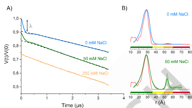
Figure 5. A) Experimental Q-band DEER traces recorded at 60 K for FMNH*/K668 pAzPhe* in absence (blue line) or in presence of NaCl 50 mM (green line), 250 mM (orange line). The black dashed lines indicate the baseline used for background correction. DEER traces were shifted vertically for the sake of clarity. B) Distance distributions obtained using the auto-computed mode in DeerAnalysis 2022 [49,50] (blue and green lines) and calculated distance distributions for the Homo sapiens CPR “locked/closed” (red line) state (pdb. 5FA6 or 3QE2) obtained using the MMM software. [48] For colour code in the x axis, see SI. [K668 pAzPhe* ] = 90 \mu M. Buffer: Tris HCl 20 mM pH 7.4, D 2 O, 10% v/v d 8 -glycerol.
