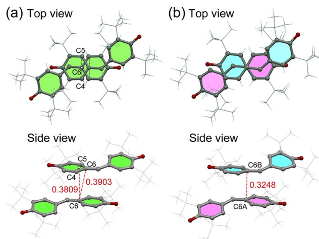
Figure 3. Nearest neighbor intermolecular arrangements in the HT (a) and LT (b) phases.
