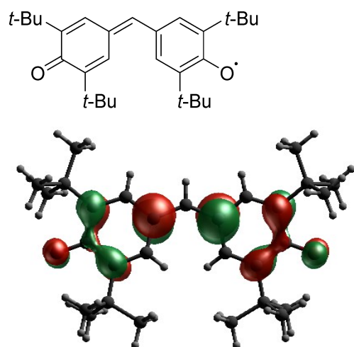
Scheme 1. Molecular structure of galvinoxyl and its SOMO calculated from a doublet CASSCF calculation.
