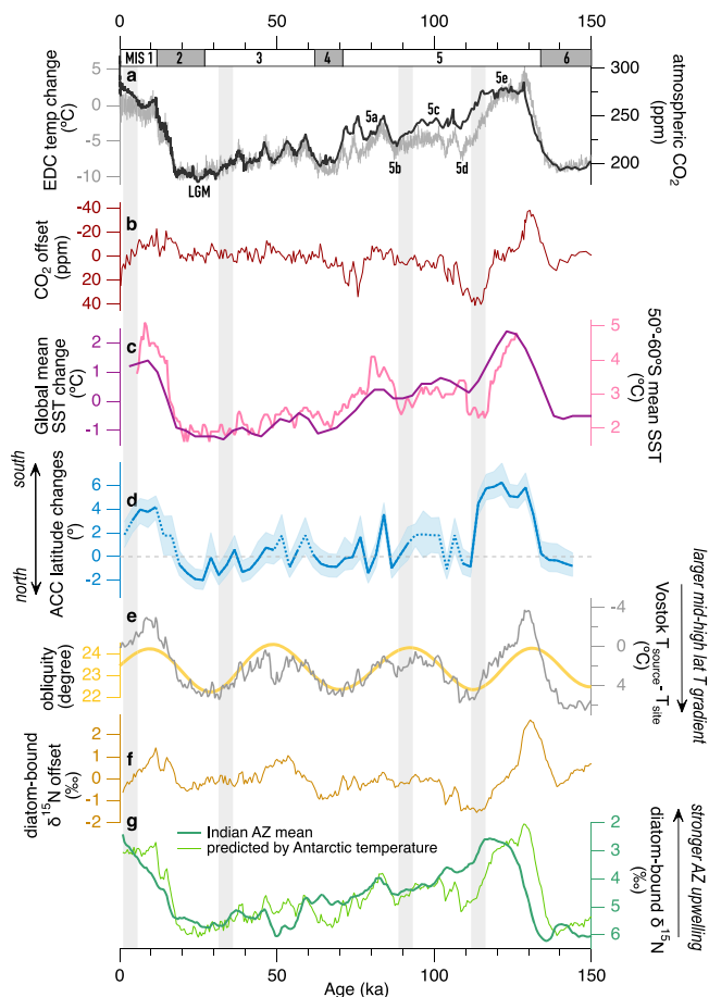
Fig. 4 Meridional migrations of the ACC over the last glacial cycle and their connections to climate and CO 2 change. a Atmospheric CO 2 72
