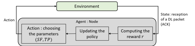
Figure 3: MAB principle applied to LoRa channel adaptation
