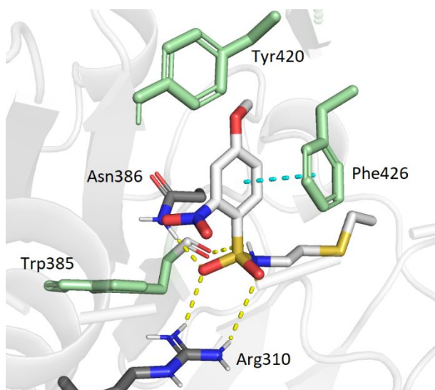
Fig. 3 Modeling docking of the best inhibitor 7 with the cap-binding pocket of SARS-CoV-2 nsp14 (PDB ID: 7R2V, resolution 2.53 Å). Contribution of the o,p -substituted arylsulfonamide core of 7 . Trp385, Tyr420, Phe426, (green), Arg310, hydrogen bonds (SO 2 – Asn386, 2.9 Å ; SO 2 – Arg310, 2.7 Å, 3.3 Å ; NH – Trp385, 2.8 Å) and the \pi - \pi stacking interaction (cyan, 4.0 Å) are shown. 5'- N -adenosine moiety is not shown for clarity purposes.
