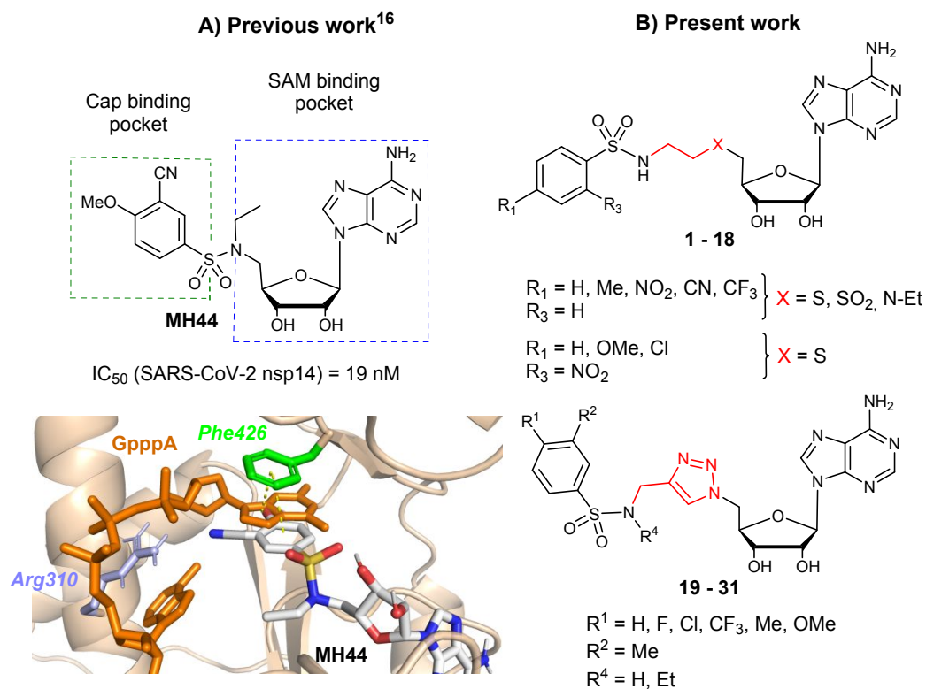
Fig. 1 A) The structure of SARS CoV-2 N7 -MTase nsp14 in which a potent inhibitor ( MH44 ) was docking into the cap-binding site of SARS-CoV nsp14 (PDB ID: 5C8S, resolution 3.3 Å) in a previous work. 23 B) Chemical structures of novel SARS-CoV-2 N7 -MTase nsp14 bisubstrates 1-31 with different linkers between the N -arylsulfonamide moiety and adenosine
