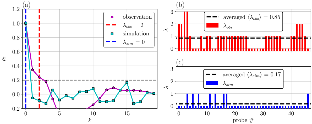
Figure 5: (a) Example of auto-correlation function vs. discrete time-lag k of the concentration sub-averages over 10 s, for both measured and simulated concentration at tower D at z = 2 m. Vertical dashed lines correspond to the correlation length (in red for measurements and in blue for simulations). (b,c) Correlation lengths computed at every probe location for measurements (in red) and simulation sub-averages (in blue). Horizontal black dashed lines correspond to the averaged correlation length over all the probes
