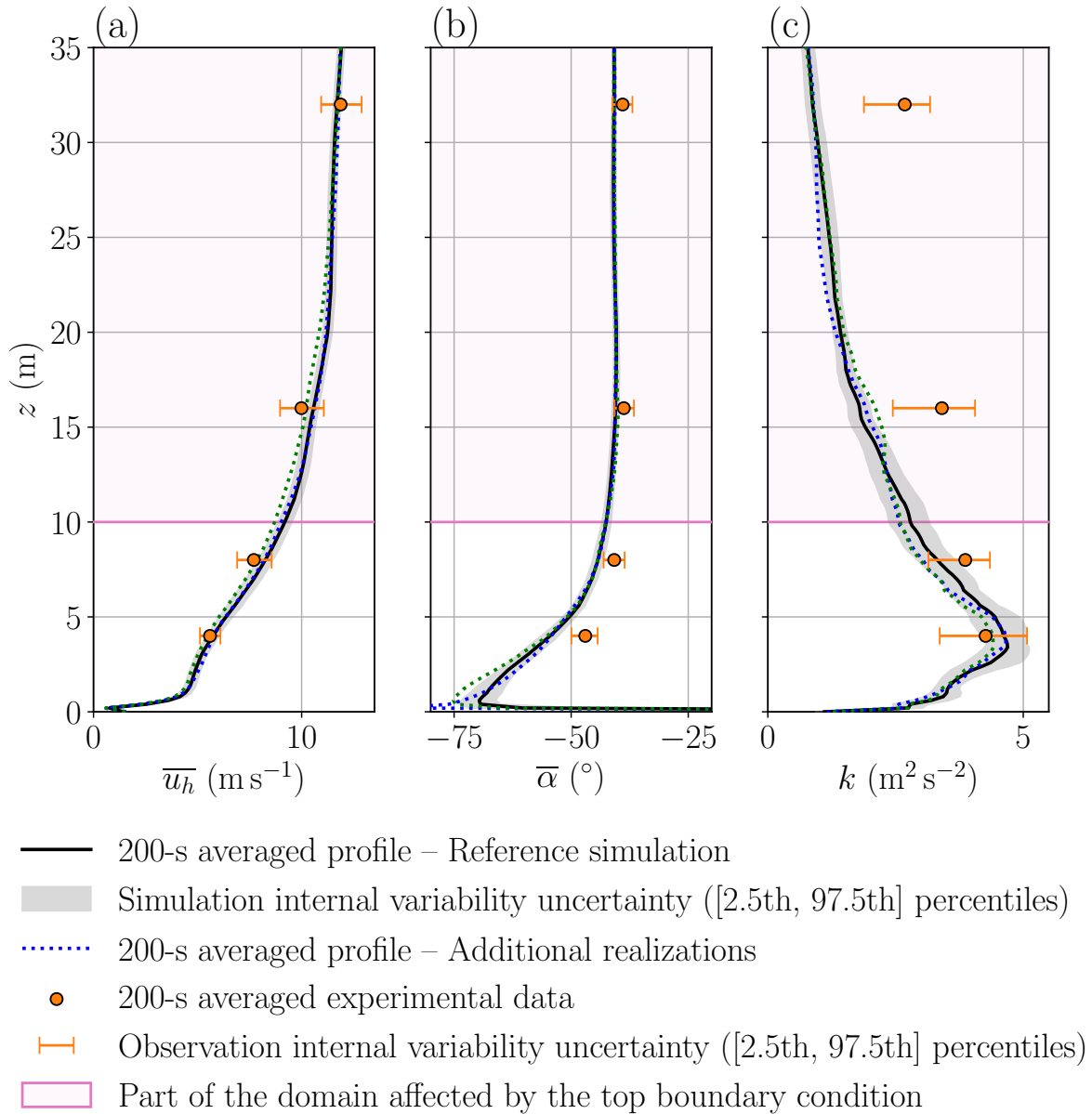
Figure 8: Vertical profiles of (a) mean horizontal wind velocity ( \text{m s}^{-1} ), (b) mean wind direction ( ^\circ ), and (c) turbulent kinetic energy k ( \text{m}^2 \text{s}^{-2} ) at the central tower T (Fig. 1). Available experimental data are represented by circles, black solid lines correspond to the LES time-averaged profiles (two additional realizations of LES estimations over 200 s are also represented as coloured dotted lines). Shaded grey areas correspond to the uncertainty induced by LES internal variability and are estimated by stationary bootstrap (the counterpart for the experimental data is indicated as error bars). The part of the domain affected by the top boundary condition according to Calaf et al. (2011) is indicated as a pink shaded area
