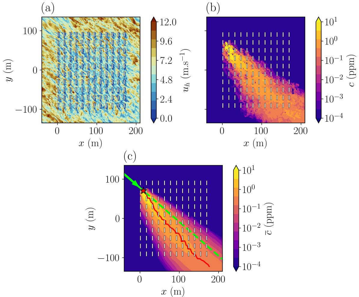
Figure 3: Horizontal cuts at z = 1.6 m of instantaneous (a) horizontal wind speed magnitude u_h ( \text{m.s}^{-1} ) and (b) propylene concentration c (ppm) at t = 60 s. (c) Horizontal cut of the time-averaged concentration over the 200-s analysis period. White rectangles represent containers. The red star represents the tracer source, and the green line represents the mean wind direction imposed at the inlet. The plume centerline, identified by the positions of the mean concentration maximum on lines orthogonal to the incident wind angle, is represented as a red line (c)
