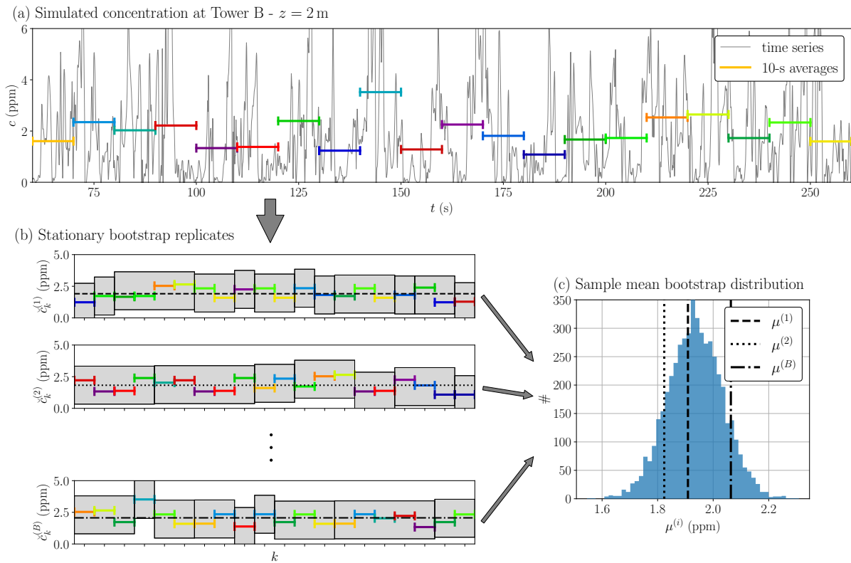
Figure 6: Stationary bootstrap algorithm applied to LES average concentration estimation at tower B ( z = 2 m). (a) Sub-averages \check{c}_k over 10 s (coloured bars) are computed over the 200-s simulated time series (grey solid line). (b) Three examples of bootstrap replicates generated by resampling with repetition of blocks of the original 10-s sub-averages, their sample means \{\mu^{(1)}, \mu^{(2)}, \mu^{(B)}\} (Eq. 11) are shown as horizontal lines and illustrate the variability induced by the resampling. (c) The statistical distribution of the sample mean estimator \mu is inferred from the B bootstrap replicates. The three examples of bootstrap realizations of time-averages of concentration over 200s \{\mu^{(1)}, \mu^{(2)}, \mu^{(B)}\} are also represented as vertical dashed lines (c). In this example, the mean block length is \ell = 2.5
