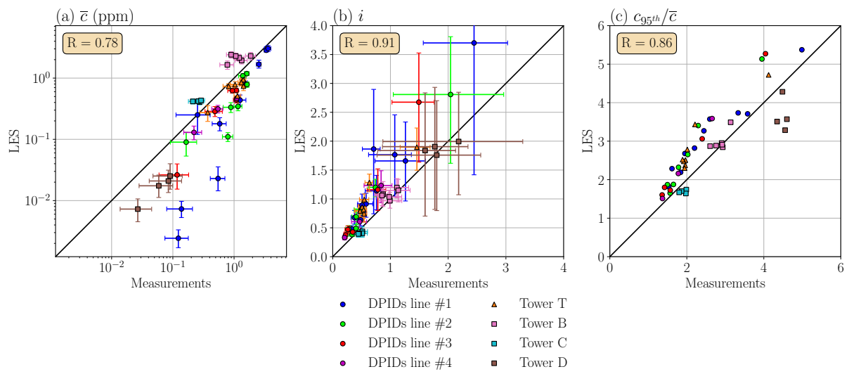
Figure 11: Scatter plots of simulated versus measured concentration statistics: (a) temporal mean, (b) fluctuation intensity, (c) normalized 95th percentile at each sensor over the detection threshold. Each type of sensor is represented with the same colour as in Fig. 1. The correlation coefficient R is indicated for each statistic. The error bars represent the 95% confidence intervals estimated through stationary bootstrap and account for the sampling error of both simulated and measured statistics (error bars are not given for the concentration maximum as the bootstrap procedure is not suitable for this statistic)
