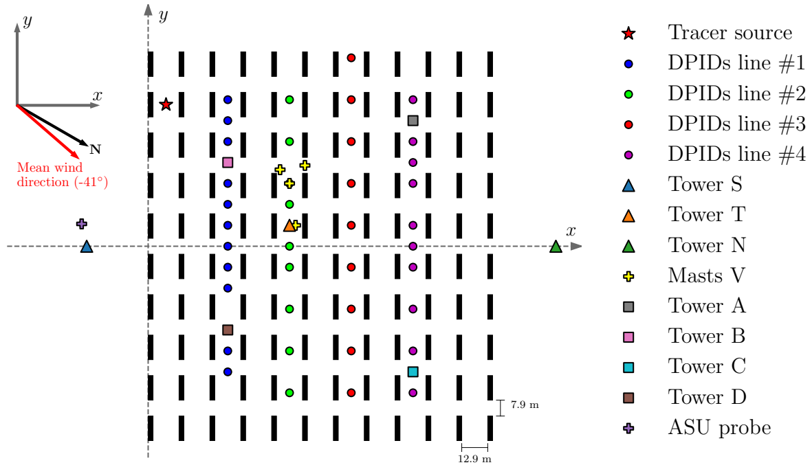
Figure 1: Schematic view of the MUST array configuration adapted from Kumar et al. (2015), the coordinate system used is the same as in Yee and Bilotft (2004) such that north corresponds to the angle of -30^\circ in the x - y coordinate system. Black rectangles represent the shipping containers used to mimic the urban canopy. Triangles correspond to the anemometers mounted on towers S, T, and N. Yellow plus symbols correspond to the masts V equipped with WDTC anemometers, and the purple plus symbol to the ASU anemometer. Coloured circles correspond to the DPID concentration samplers (one colour for each line of sensors), and coloured squares correspond to the UVIC concentration samplers mounted on towers A, B, C, and D (note that there is a DPID sampler at the same location as tower D). The upstream mean wind direction (red arrow) and the propylene-source location (red star) of the trial 2681829 retained for the present study are also indicated
