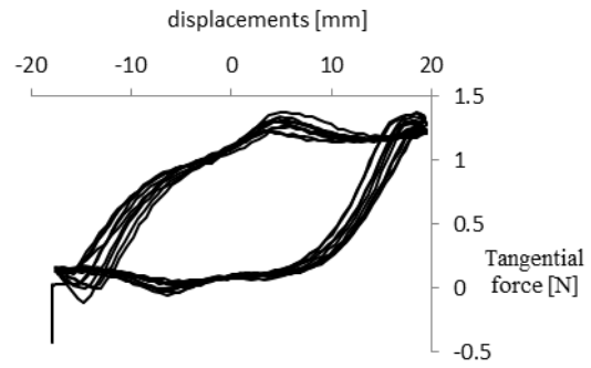
Fig. 8 – Phase plot for the dynamics of the unloaded measuring system (offset not removed).
