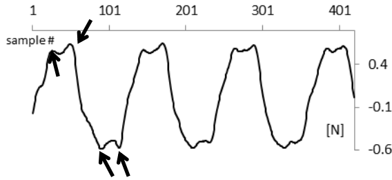
Fig. 7 – Tangent force signal (unloaded measuring system) averaged over 5 periods, with average of the signal nulled.
