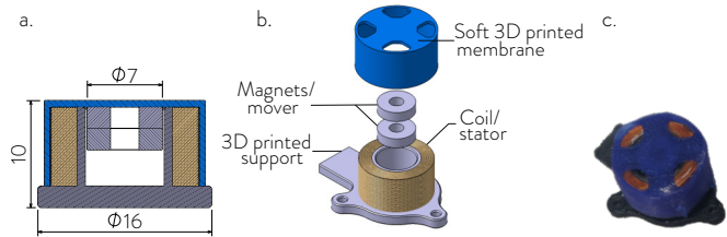
Fig. 2. Our custom-design electromagnetic actuator with the soft 3D-printed membrane. Five of these actuators are housed inside each handle (see Fig. 1). a) Cut view. b) Isometric View. c) Picture of the actuator.
