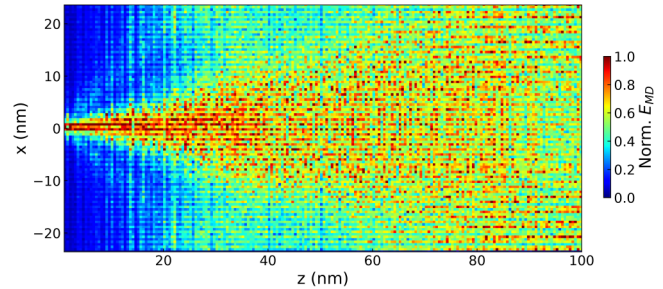
FIG. 9. Visualization of the diffraction and interference patterns created by a 6 THz continuous longitudinal plane wave going through an aperture of a width of 3 nm using a void barrier at 25 K. The energy value is normalized by the maximum value for each pixel column along z .
