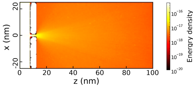
FIG. 7. Same configuration as presented in Fig. 2 simulated with the Monte Carlo method.
