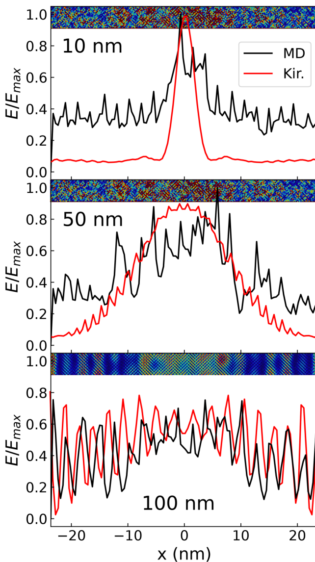
FIG. 5. Kinetic energy distribution along the x axis at z = 10, 50, and 100 nm of the MD simulation with an a-Si barrier (full black line) and the Kirchhoff model in red. The insets give an atomic representation of the same quantity with the same color scale as Fig. 2 (blue is zero and red is 2 \times 10^{-09} eV/atom).
