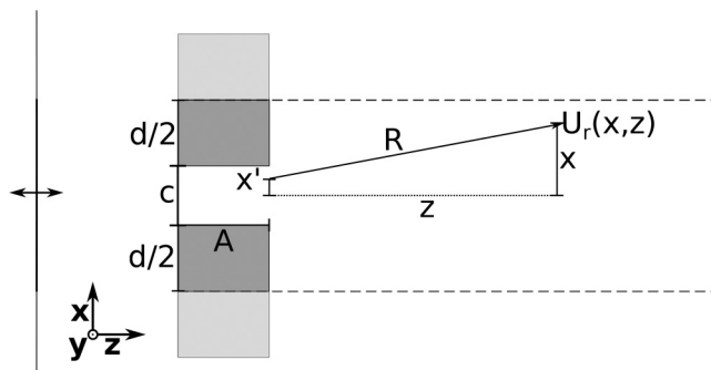
FIG. 1. Schematic representation of the system with the parameters used for Eq. (1), the gray area represents the barrier (void or a-Si), the dashed lines show the periodic boundary condition, and the vertical line with an arrow is the zone where phonons are excited.
