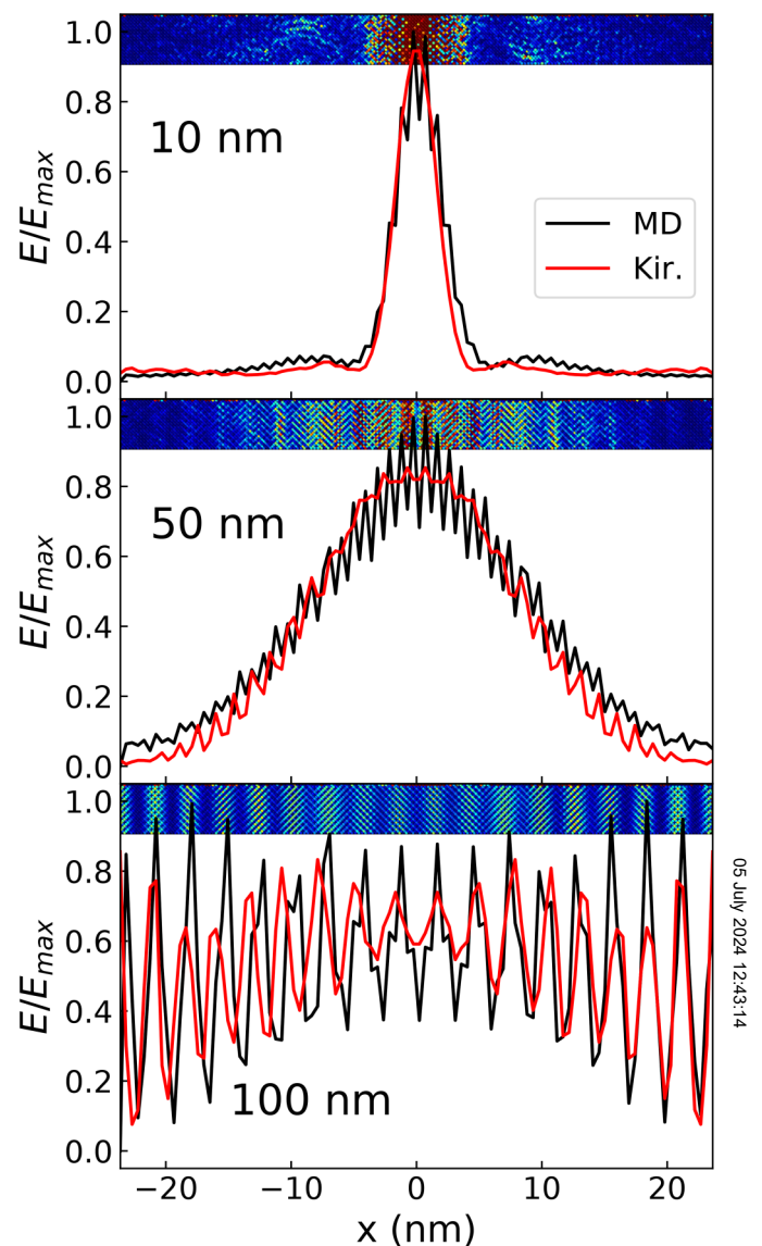
FIG. 4. Kinetic energy distribution along the x axis at z = 10, 50, and 100 nm of the MD simulation with a void barrier (full black line) and the Kirchhoff model in red. The insets give an atomic representation of the same quantity with the same color scale as Fig. 2 (blue is zero and red is 2 \times 10^{-09} eV/atom).
