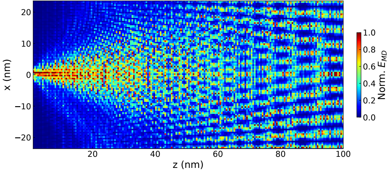
FIG. 8. Visualization of the diffraction/interference pattern caused by a 3 THz continuous transverse plane wave going through an aperture of a width of 3 nm using a void barrier. The energy value is normalized by the maximum value for each pixel column along z .
