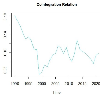
Fig. 3. Cointegration relationship plot
