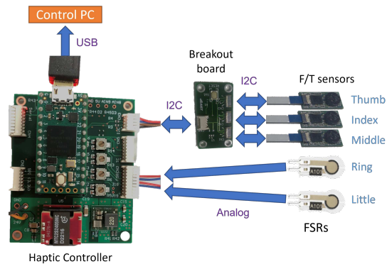
Fig. 15 Haptic system of each hand.
