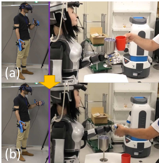
Fig. 37 Screenshots showing the execution of the toast and handshake task: (a) robot grasping the wine glass and making toast, (b) the recipient applies force to move the robot's hand to do a handshake (in this case, the operator did not move his hand, so the robot's arm showed compliance).
