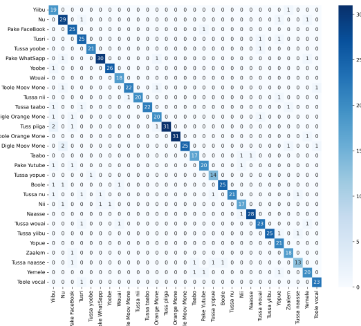
Fig. 6. RNN Confusion Matrix
