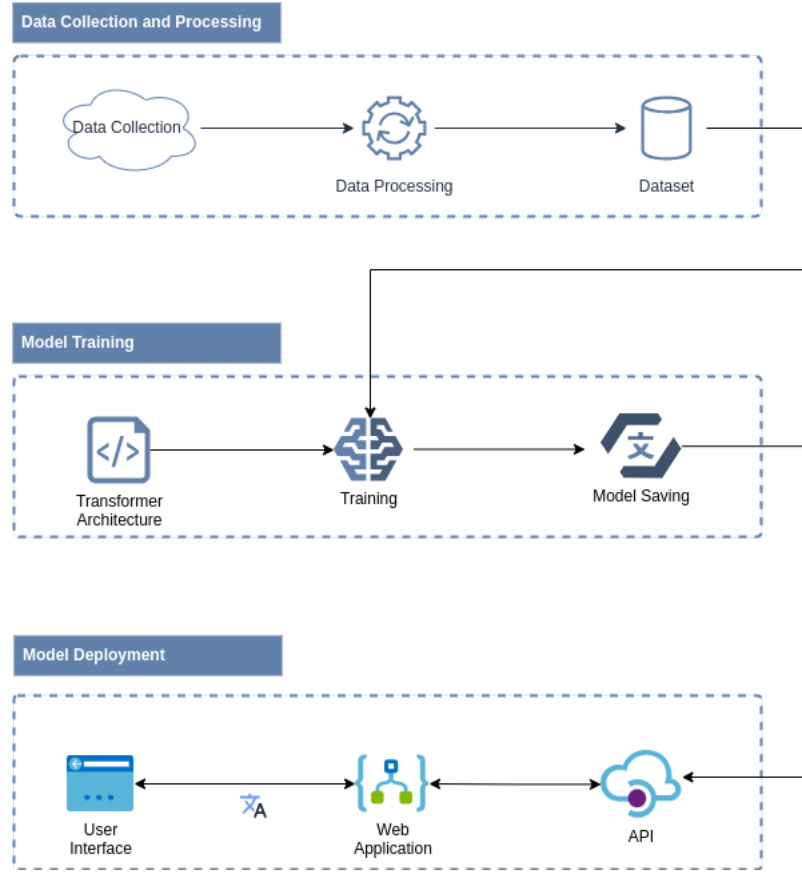
Fig. 1. Comprehensive methodology for developing a LOw-ressource language Translation system
