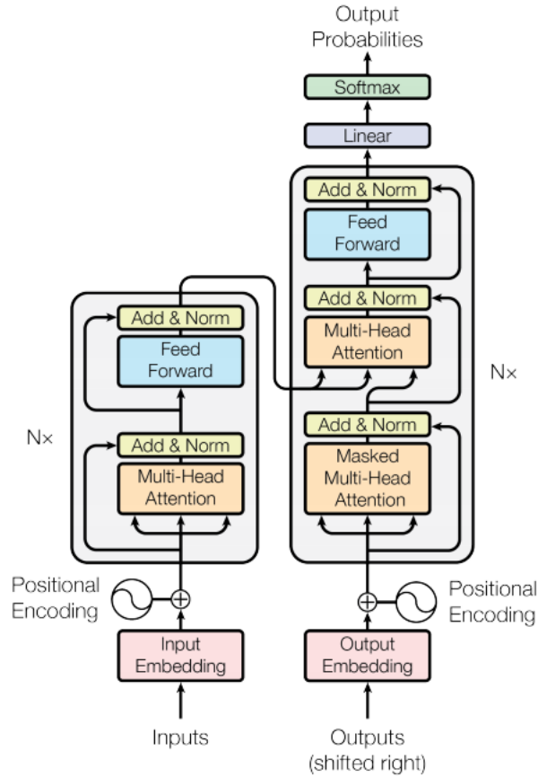
Fig. 2. Transformer Architecture
