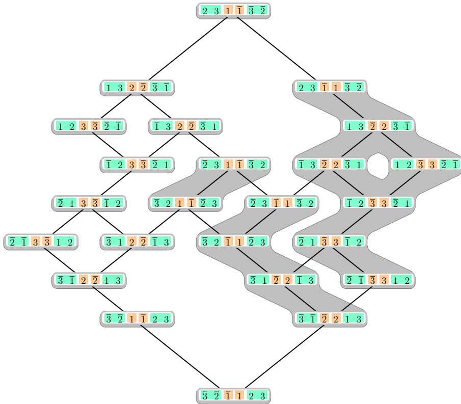
Figure 5: The weak order on \mathfrak{S}_{(0,1,2)} with the congruence classes with respect to \Theta highlighted.
