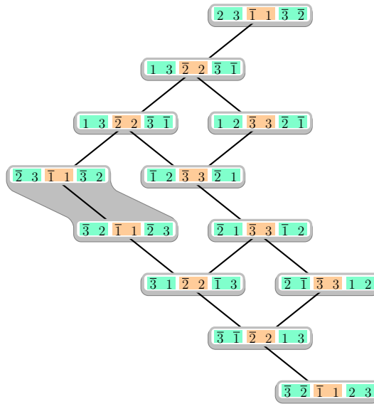
Figure 4: The weak order on \mathfrak{H}_{(1,2)} with the congruence classes with respect to \Theta highlighted.
