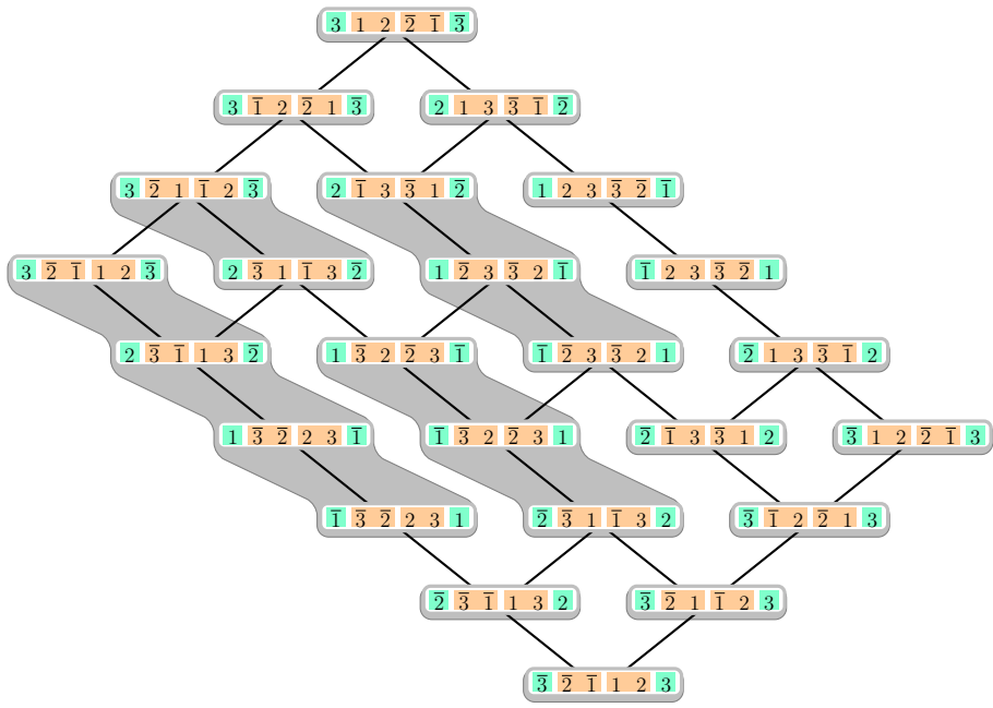
Figure 8: The weak order on \mathfrak{H}_{(0,2,1)} .
