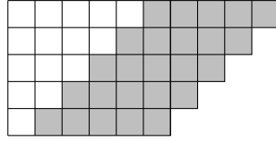
Figure 3: The skew shape \lambda/\mu , where \lambda = (10, 9, 8, 7, 6) and \mu = (5, 4, 3, 2, 1) , consists of the gray boxes.
