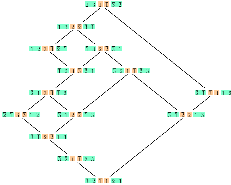
Figure 7: The lattice \text{Tam}_B((0, 1, 2)) .
