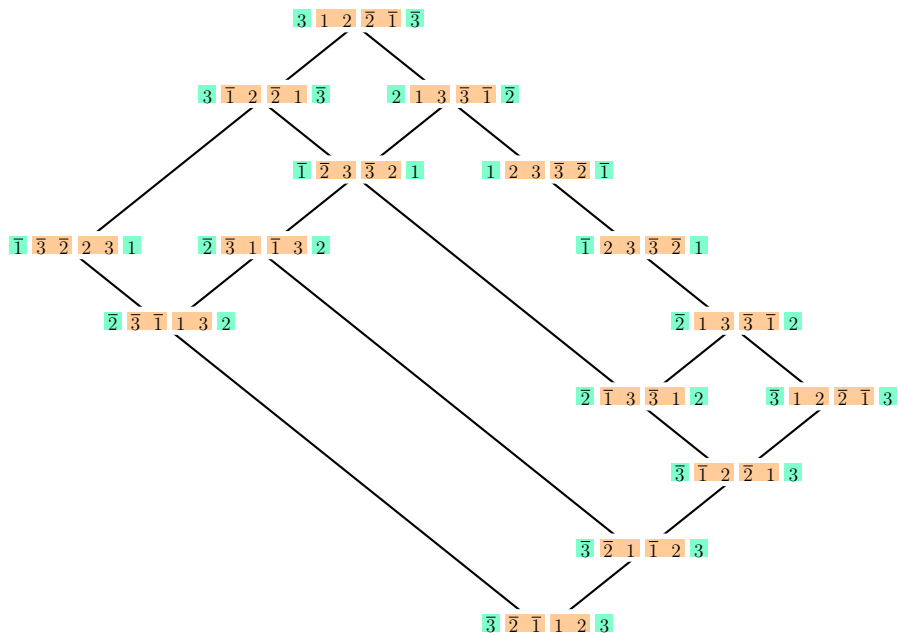
Figure 9: The lattice \text{Tam}_B((0, 2, 1)) .
