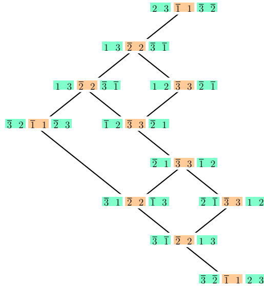
Figure 6: The lattice \text{Tam}_B((1, 2)) .
