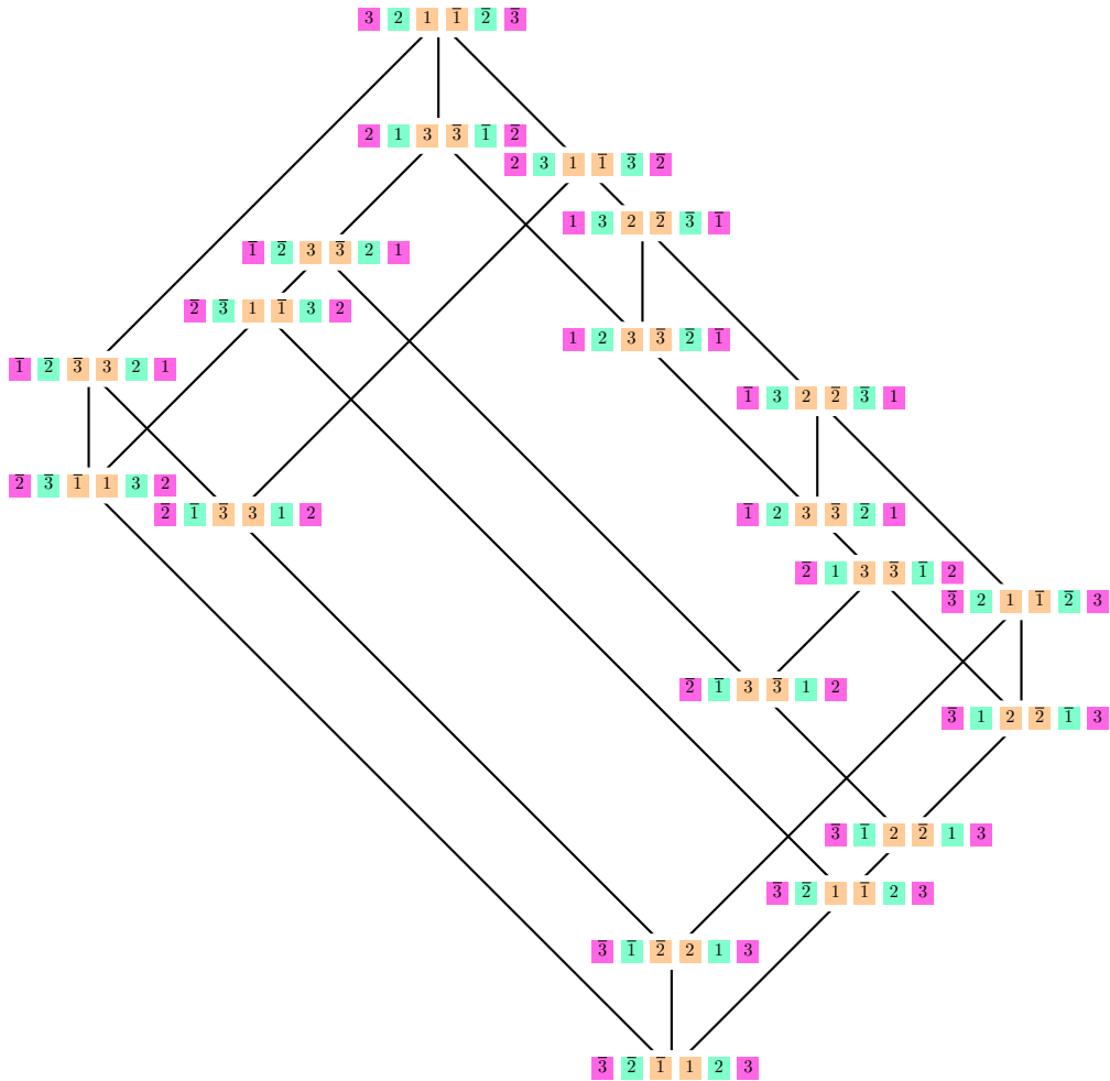
Figure 2: The lattice \text{Tam}_B(3) .
